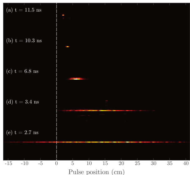
FIG. 2. Pulse compression for varying group velocity. The real time t is given for each pulse, with t = 0 ns corresponding to the time when the pulse enters the Rb vapour at z = 0 cm. The white dashed line denotes the position at which the light enters the Rb vapour. (a)-(d) correspond to group velocities of v_g = c/183 , c/81 , c/24 , and c/2.6 , with temperatures of T \sim 150, 130, 106 , and 50 °C, respectively. (e) shows the pulse propagating through air to provide a reference for light traveling at v_g \sim c . See corresponding video (supplemental information) for the full pulse propagation. A 7-cm cell was used to obtain the higher temperatures necessary for (a) and (b), while a 30-cm cell was used for (c) and (d).
