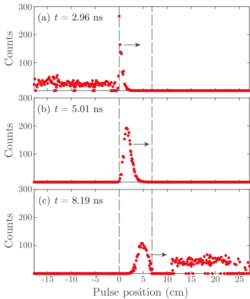
FIG. 3. Pulse compression. Subsequent frames show the pulse (a) propagating through air, (b) entering the heated Rb vapour cell ( L \sim 7 cm) and compressing spatially due to the decrease in group velocity, and (c) exiting the cell and decompressing. The arrow indicates the direction of pulse propagation. See corresponding video (supplemental information) for the full pulse propagation. Pulse amplitudes are scaled with respect to the initial pulse amplitude (initial camera position) to account for variation in pulse energy between scans.
