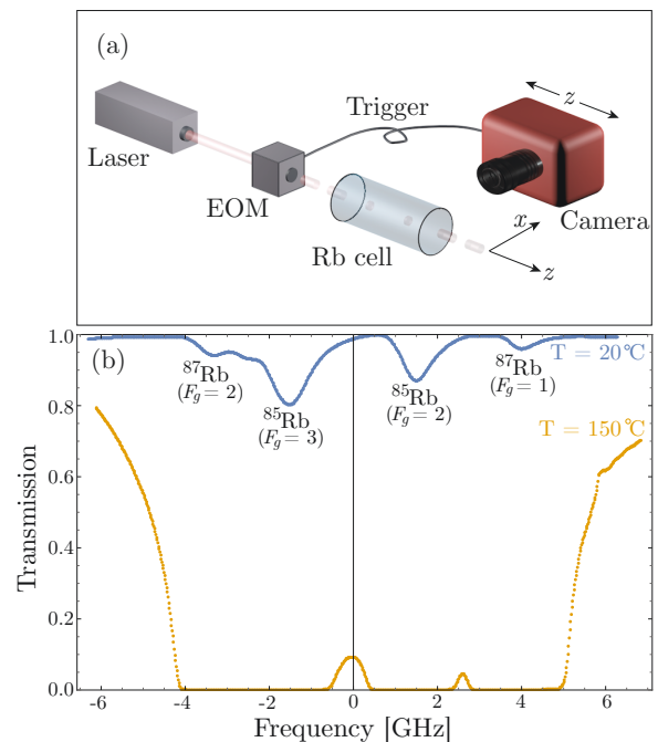
FIG. 1. (a) Experimental setup (not to scale). The EOM chops the laser beam into pulses, which propagate through the Rb vapour cell, from left to right along the z axis. The SPAD camera is set up to capture light scattered by the Rb vapour along the x axis. The camera has a 5-cm field of view (resolution of \delta z = 1.6 mm) and is scanned along the z axis by 4-cm increments. (b) Transmission spectra for the L = 7.18 cm cell. A temperature of T \sim 150^\circ\text{C} corresponds to an OD \sim 2.5 at \delta \sim 0 GHz, with a group velocity v_g = c/183 , determined from the SPAD data. The room temperature transmission spectrum, T \sim 20^\circ\text{C} , is provided for reference.
