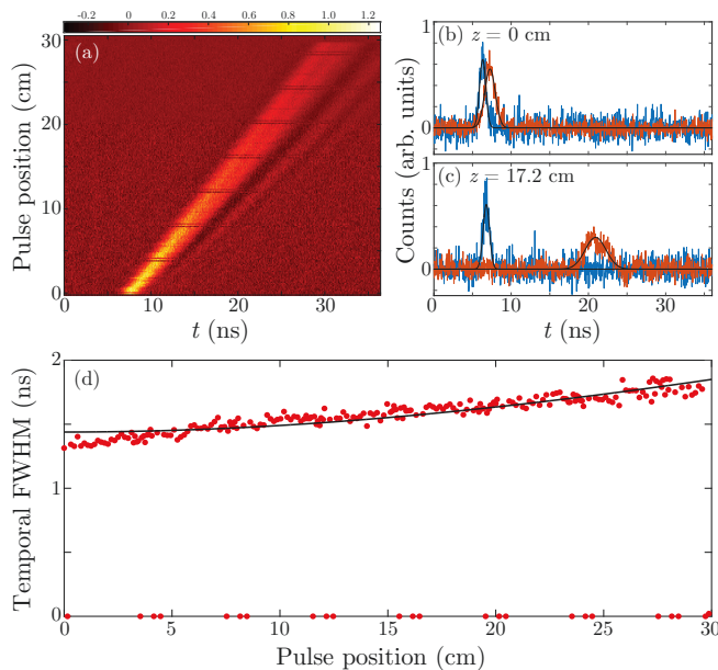
FIG. 5. Pulse dispersion observed for a pulse propagating through a Rb vapour cell of length L = 30 cm, with v_g \sim c/24 ( T \sim 104^\circ\text{C} ). (a) Plot of raw pulse temporal profiles (horizontal axis) for increasing propagation distance z (pulse position, vertical axis). (b)-(c) Raw histograms and Gaussian fits to the temporal pulse profiles for z = 0 cm and z = 17.2 cm, respectively ( z = 0 cm corresponds to the temporal pulse profile directly after it enters the Rb vapour). Blue traces correspond to a pulse in air for comparison. Relative amplitudes have been scaled (air: N_{\text{counts}}/70 , Rb: N_{\text{counts}}/200 ) to allow for a comparison of the pulse shape. (d) Representative plot of pulse temporal FWHM \tau versus pulse position z (red circles) for T \sim 100^\circ\text{C} , OD \sim 0.63 and v_g \sim c/13 . Solid black line: data fit with the function \tau(z) = \sqrt{\tau_0^2 + (Bz/\tau_0^2)^2} , where \tau_0 = 1.44 ns is the pulse FWHM width at z = 0 and \beta_3 = B/\sqrt{16(\ln(2))^3} = 0.035 ns 3 /cm. Noisy pixels, corresponding to the repeating line artefacts observed in (a), are set to \sigma = 0 and excluded from the fit shown in (d).
