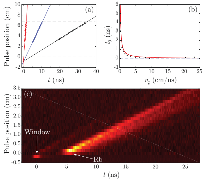
FIG. 4. (a) Representative plots of pulse position along the beam path z versus the scattered photon arrival time t , shown for group velocities v_g \sim c/6 (red squares), v_g \sim c/41 (blue circles) and v_g \sim c/139 (black diamonds). Horizontal dashed lines denote the inner edges of the Rb vapour cell, where z = 0 corresponds to where the pulse enters the Rb vapour. Solid lines are fits z = v_g(t - t_0) to the data. (b) Photon-lag time versus group velocity. Black circles: extrapolated time t_0 at which the light entered the Rb vapour versus v_g . Red solid line: calculated time lag t_0 = r_{\text{cell}}/v_g , where r_{\text{cell}} = 1.175 cm is the inner radius of the vapour cell. Blue dashed line: time lag t_0 = r_{\text{cell}}/c = 0.04 ns that one would expect if the scattered photons traveled out of the medium at c . (c) Raw temporal profiles corresponding to each pulse propagation position for v_g \sim c/183 . Note that the light scattered just after the pulse enters the Rb vapour arrives at the camera approximately 5.3 ns later than the light scattered by the glass window (indicated by white arrows).
