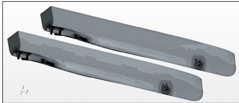
Figure 5. Grid structure on the fully-apped Stavanger Demonstrator.
