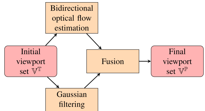
FIGURE 3. Overview diagram of Viewport Prediction Hybrid (VPredHYB).
