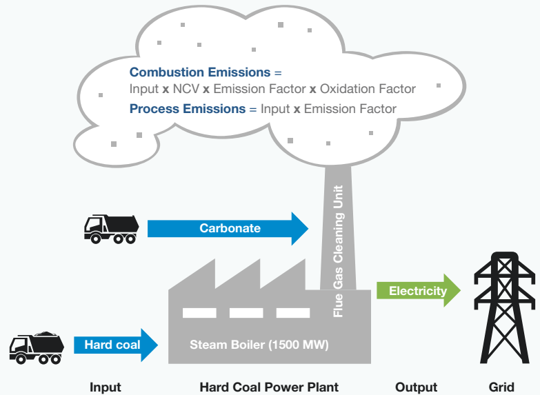
Figure 7-5 Simplified example of annual emissions monitoring (calculation) in a hard coal power plant
