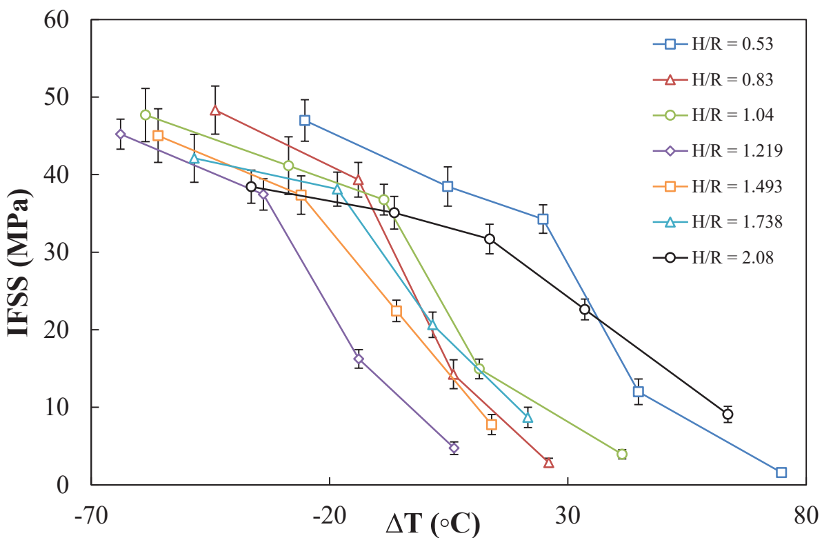
Fig. 9. Plot of IFSS versus \Delta T , where \Delta T = T_t - T_g for APS fibres.
