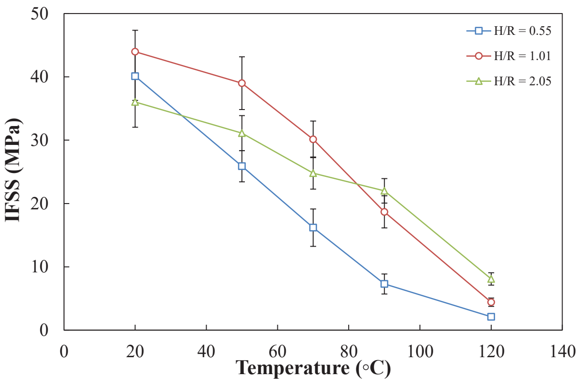
Fig. 10. Plot of IFSS versus Testing Temperature for GPS fibres.
