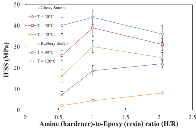
Fig. 11. Plot of IFSS versus amine (hardener)-to-epoxy (resin) ratio (H/R) for GPS fibres.
