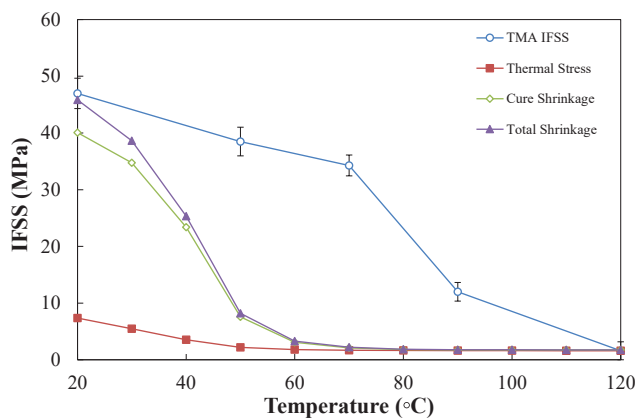
Fig. 15. Comparison of glass fibre epoxy IFSS with calculated residual radial stresses for an amine (hardener)-to-epoxy (resin) ratio of H/R \approx 0.5 .
