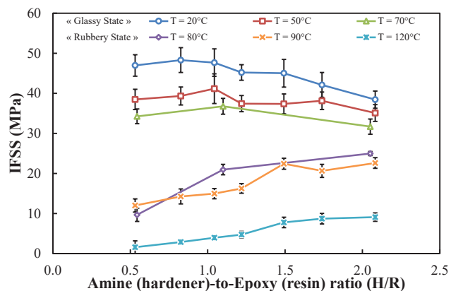
Fig. 8. Plot of IFSS versus amine (hardener)-to-epoxy (resin) ratio (H/R) for APS fibres.
