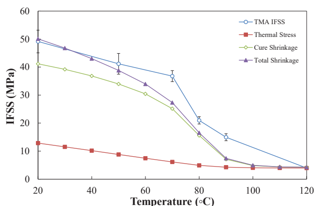
Fig. 20. Comparison of glass fibre epoxy IFSS with adjusted residual radial stresses for an amine (hardener)-to-epoxy (resin) ratio of H/R \approx 1.0 (the stoichiometric value) using a coefficient of static friction = 0.75.
