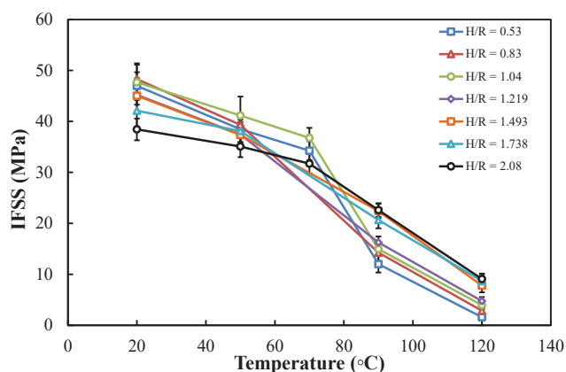
Fig. 7. Plot of IFSS versus Testing Temperature for APS fibres.
