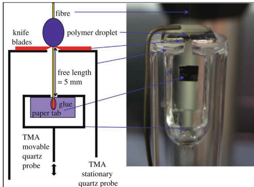
Fig. 1. Schematic and close up photograph of TMA-Microbond test setup [15].
