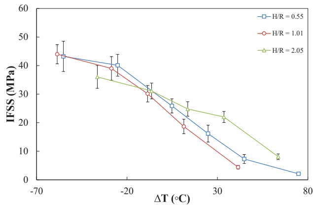
Fig. 12. Plot of IFSS versus \Delta T , where \Delta T = T_t - T_g for GPS fibres.
