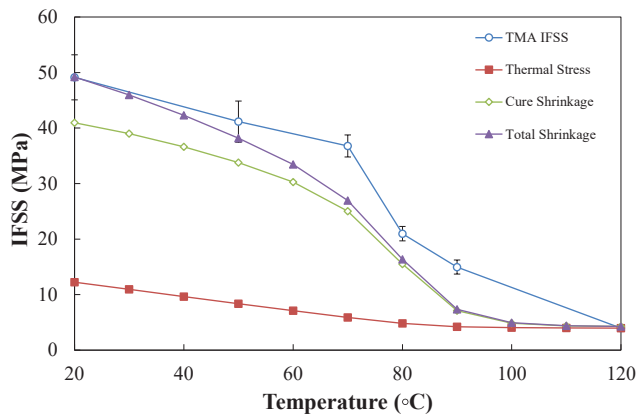
Fig. 14. Comparison of glass fibre epoxy IFSS with calculated residual radial stresses for an amine (hardener)-to-epoxy (resin) ratio of H/R \approx 1.0 (the stoichiometric value).
