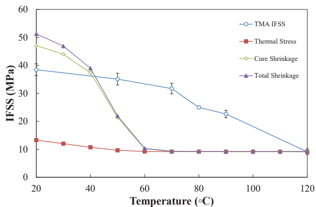
Fig. 16. Comparison of glass fibre epoxy IFSS with calculated residual radial stresses for an amine (hardener)-to-epoxy (resin) ratio of H/R \approx 2.0 .
