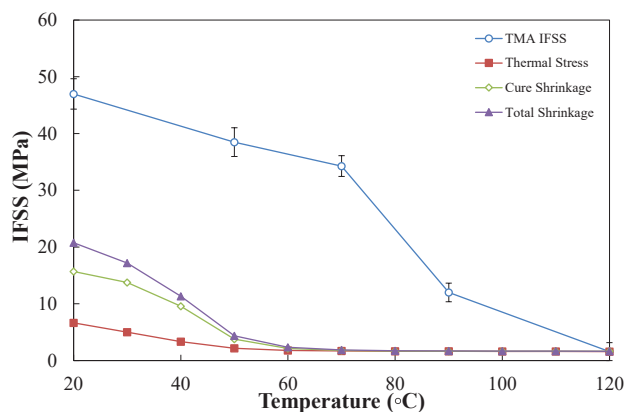
Fig. 18. Comparison of glass fibre epoxy IFSS with adjusted residual radial stresses for an amine (hardener)-to-epoxy (resin) ratio of H/R \approx 0.5 .
