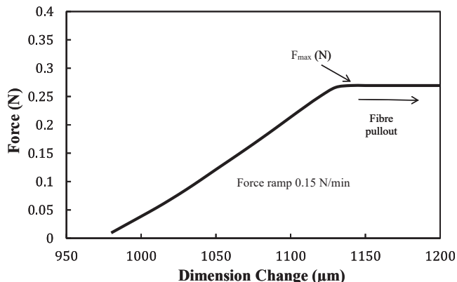
Fig. 2. Load/ Displacement Curve for TMA microbond test.
