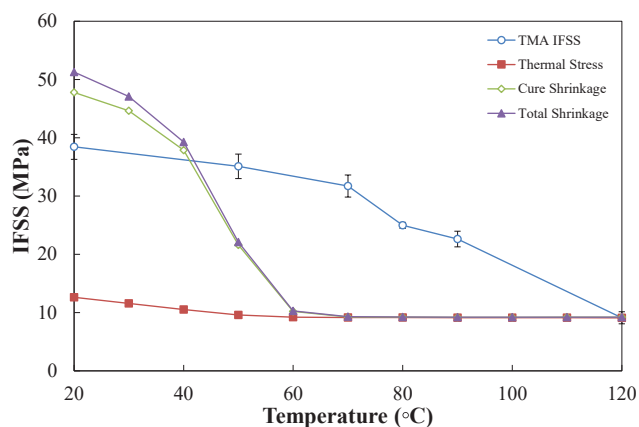
Fig. 19. Comparison of glass fibre epoxy IFSS with adjusted residual radial stresses for an amine (hardener)-to-epoxy (resin) ratio of H/R \approx 2.0.
