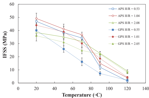
Fig. 13. Plot comparing results for H/R \approx 0.5 , H/R \approx 1.0 and H/R \approx 2.0 for both silanes studied.
