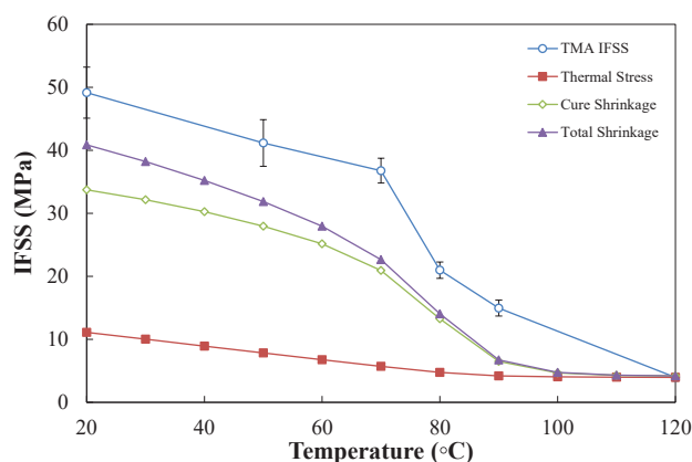
Fig. 17. Comparison of glass fibre epoxy IFSS with adjusted residual radial stresses for an amine (hardener)-to-epoxy (resin) ratio of H/R \approx 1.0 (the stoichiometric value).
