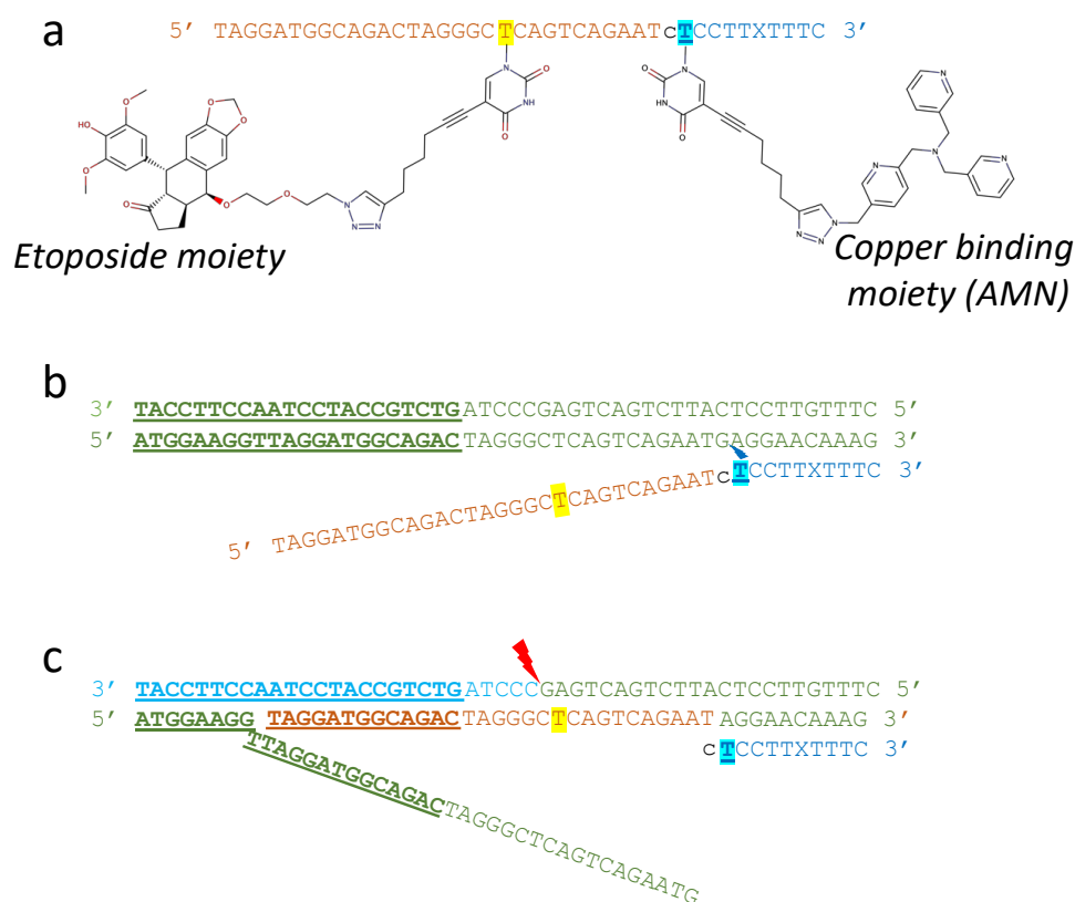
Figure 5. A 41 mer comprising a 30 mer etoposide-OTI coupled to a 10 mer AMN-TFO. (a) Depiction of a 41 mer, in which a 30-mer WC-OTI (orange letters with etoposide attached to yellow highlighted T) has been linked (single c in black) to a ten nucleotide TFO (blue letters) with a copper binding artificial
