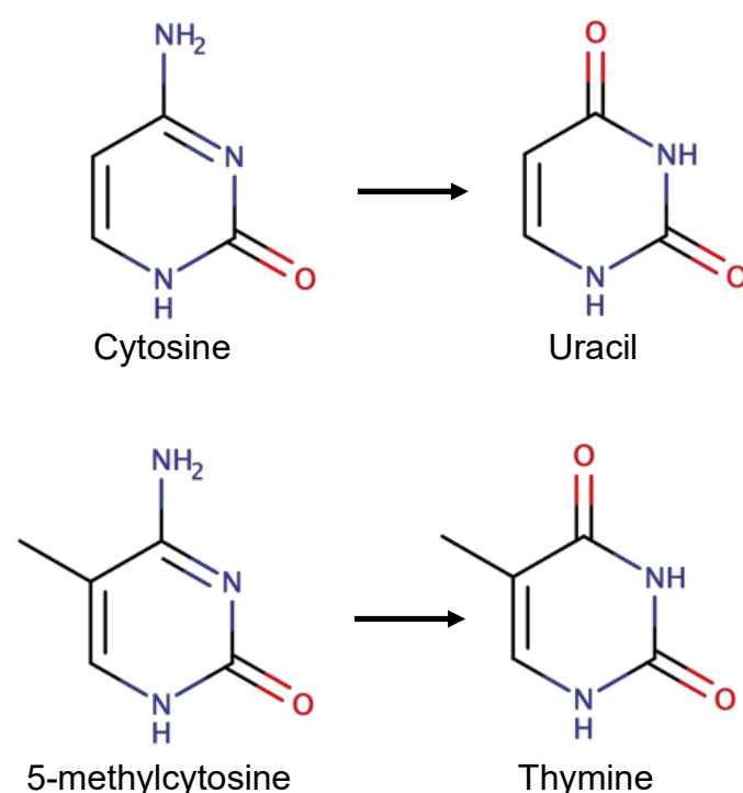
Figure 6. Deamidation of cytosine to uracil and 5-methylcytosine to thymine. The exocyclic amine of cytosine can be spontaneously deamidated to give uracil and the exocyclic nitrogen of 5-methylcytosine can be spontaneously deamidated to give thymine. Uracil is removed from DNA by uracil-DNA glycosylase while the G:T base-pair resulting from spontaneous deamidation of 5-methylcytosine can be removed by thymine DNA glycosylase (Figure drawn with Marvin-Sketch, from ChemAxon, https://www.chemaxon.com ).
