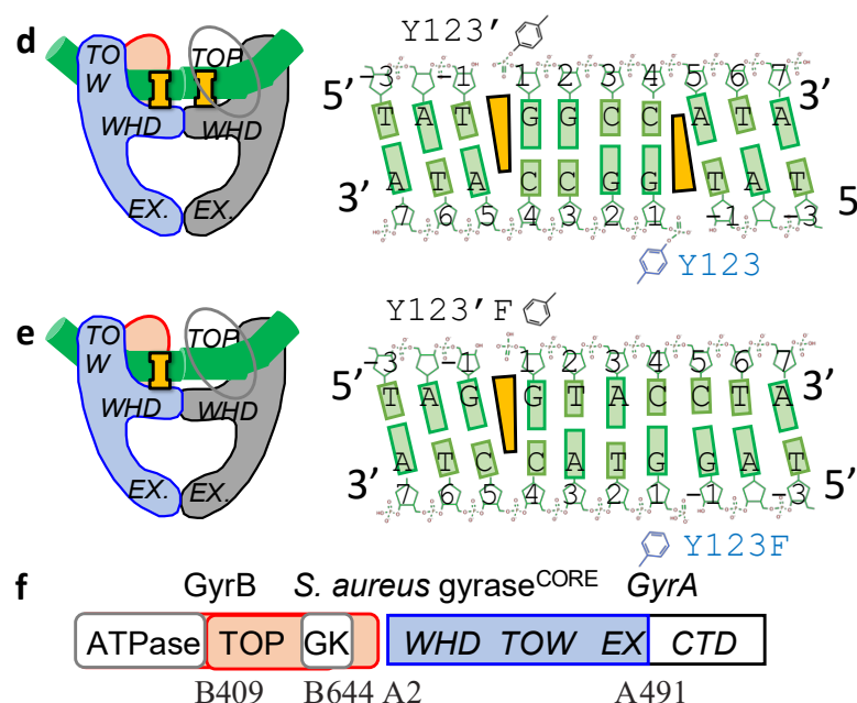
Figure 3. Type IIA topoisomerases and schematics of three etoposide crystal structures. (a) Simplified schematic of a reaction carried out by a type IIA topoisomerase. The gate or G-DNA (green cylinder) is cleaved and another DNA duplex, the T (or transport segment; black) is passed through the cleaved DNA before religation. (b) Schematic of a 2.16 Å human hTOP2β core structure (pdb code: 3qx3) with DNA and two etoposides (I) binding at the two DNA cleavage sites, four base-pairs apart. One subunit is shown in red and blue, the other in grey. The DNA sequence (5'-3') is the same for both strands; the DNA has been cleaved by tyrosine 821. (c) In human TOP2β is a single subunit and functions as a homodimer; the hTOP2β core is residues 445-1201. Structural domains in hTOP2β core are TOPRIM (TOP) domain, GK = Greek key domain, WHD = winged helical domain, TOW = tower domain, EX = exit gate domain. (d) Schematic of a 2.8 Å structure of S. aureus gyrase core fusion truncate DNA complex containing two etoposide (I) binding at the two DNA cleavage sites (pdb code: 5cdn), four base-pairs apart. One gyrase core fusion truncate is shown in red and blue, the other in grey. (e) Schematic of a 2.45 Å structure of S. aureus gyrase core fusion truncate DNA complex containing one etoposide (I) (pdb code: 5cdp). (f) DNA gyrase consists of two subunits, GyrB and GyrA (domains are indicated). Note in the S. aureus gyrase core fusion truncate the GyrB and GyrA subunits are fused into a single 'subunit' (B409-B644 + A2-A491) and the small greek key domain (residues B544-B579) has been deleted.
