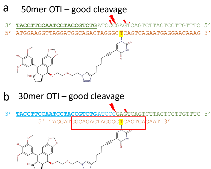
Figure 4. 50 mer and 30 mer Watson–Crick-OTIs cleave an oncogene target sequence. Adapted from Figure 9 in [43] focusing on Top2 \alpha cleavage. (a) The target oncogenic PML-RARA sequence to be cleaved is shown in green on the top line, with the RARA sequence bold and underlined at the 3' end; the 5' sequence is from PML. The bottom line shows the 50 mer OTI with an etoposide moiety covalently attached to the T (highlighted in yellow). DNA-cleavage gels showed that the OTI promoted DNA-cleavage at four sites on the target (green) strand with relative intensities (in brackets) 24–25 (17), 23–24 (45), 20–21 (17), 19–20 (5). (b) The same target PML-RARA sequence is shown on the top line, but coloured in cyan at the 3' end to indicate the position of the major cleavage site. Only two DNA-cleavage sites were observed with the 30 mer OTI, 23–24 (32), 20–21 (9) (red lightning bolts show positions). The red box indicates where the 20 nucleotides are from Xtal structures with etoposide (pdb codes: 3qx3, 5cdn and 5cdp);–based on the major DNA-cleavage site.
