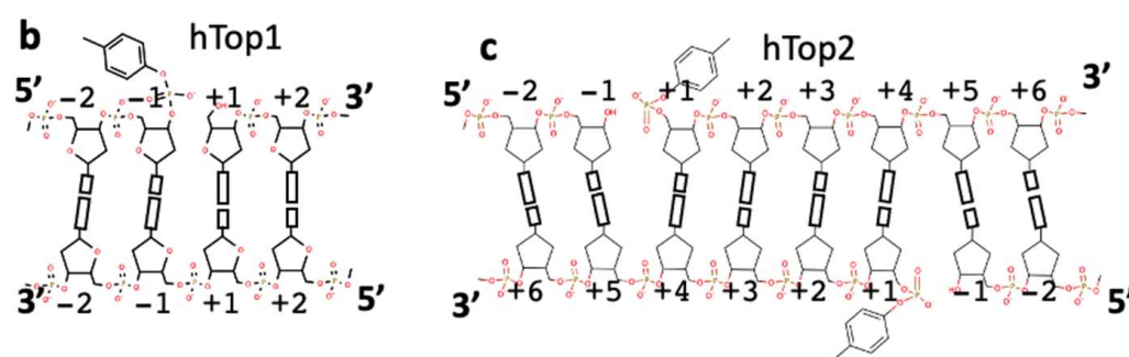
Figure 1. Human Top1 and Top2 regulate DNA topology at a transcription bubble. (a) In the post-mitotic cells of the central nervous system-human Top1 and human Top2 \beta are expected to be active in regulating DNA topology near transcription bubbles. The only DNA replication in post-mitotic CNS cells will take place in mitochondria; and careful design may be needed to ensure that damage to replicating mitochondrial DNA does not take place [27]. RNAPII, RNA polymerase II, is shown in contact with Top1 [28]. (b) Human Top1 cleaves a single DNA strand forming a 3' phosphotyrosine. By convention both cleaved and non-cleaved strands are numbered relative to the single DNA-cleavage site. (c) Human Top2 (Top2 \alpha or Top2 \beta ) can cleave both DNA strands forming two 5' phosphotyrosines. By convention both strands are numbered relative to the two 4-base-pair staggered DNA-cleavage sites.
