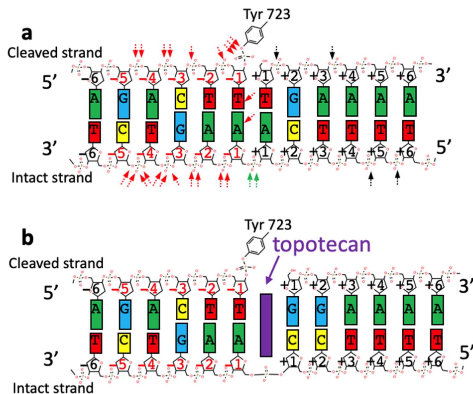
Figure 2. Simplified schematics of twelve base-pairs of DNA in TOP1 DNA-cleavage complexes. (a) Simplified schematic of the central twelve base-pairs of DNA in a Top1 DNA-cleavage complex (based on 2.1Å structure pdb code: 1a31). Interactions (<3.5Å) between the protein and the DNA are represented by arrows (adapted from Figure 4, panel G in [59]). Tyrosine 723 from Top1 has cleaved the top strand. Top1 can be imagined as a hand holding the double-stranded DNA up-stream of the DNA-cleavage site (red arrows and–red numbered nucleotides) and allowing controlled rotation about the phosphodiester bond between the –1 and +1 nucleotides on the intact strand (two green arrows) to relax the DNA. (b) A simplified schematic of the same DNA sequence in a complex with topotecan (a camptothecin derivative). The figure is based on the 2.1Å structure with topotecan (pdb code 1K4T). Note the +1 G–C base-pair (in 1K4T). The topotecan occupies the ‘same’ space as the +1 nucleotide pair in panel a. ‘The intercalation binding site is created by conformational changes of the phosphodiester bond between the +1 and –1 base pairs of the intact strand’ [45].
