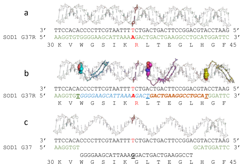
Figure 7. Modelling a theoretical correction by three camptothecin based PIP-OTIs of a mutation associated with familial ALS. (a) A model (BDNA, 8 June 2022, from http://www.scfbio-iitd.res.in/software/drugdesign/bdna.jsp ) of nucleotides (one strand carbons in black, the other in green) coding amino acids 30–45 (single letter code bottom line) of human SOD1 with a G37R mutation. The single base-pair change causing the glycine to arginine mutation is highlighted in red. (b) Three camptothecin based PIP-OTIs are shown coloured with cyan, magenta and yellow carbons, with the intercalating camptothecin moiety in solid space-fill representation. Three positions ( I G) cut on the lower strand, in the presence of Top1 (see also Supplementary Figures S3 and S5) are indicated. In cleavage complexes the T is covalently bonded to Top1 by a 3' phosphotyrosine bond and the camptothecin moiety intercalates between the T A and GC base-pairs at the DNA-cleavage site. (c) The blue and orange oligonucleotides in b are envisioned to have been removed – and are replaced with an oligonucleotide with a corrected G . The T in the central G-T mismatch should be removed by thymine DNA-deglycoylase–after which the red T in the top strand should be corrected to C.
