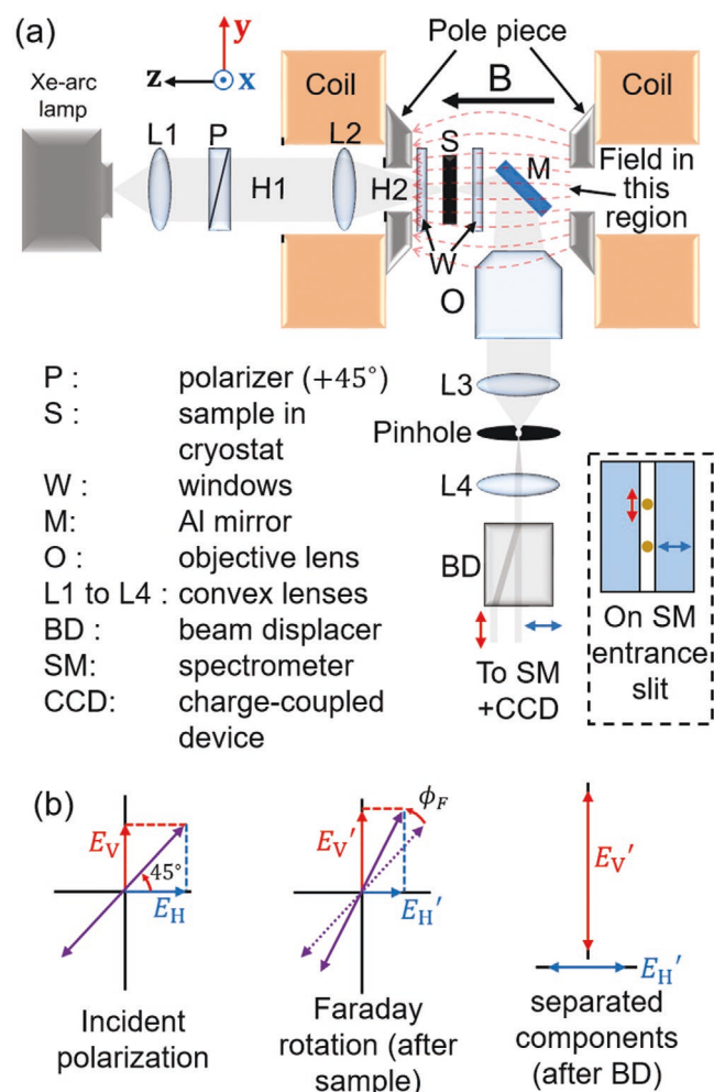
Figure 1. Schematic of the Faraday rotation spectroscopy setup. a) Schematic (top view) of the Faraday rotation spectroscopy setup depicting the arrangement of the key components. The inset (dashed lines) shows the focused spots corresponding to the two polarization components split by the beam displacer (BD) at the entrance slit of the spectrometer (SM). b) Polarization state of the light after passing through the sample and the beam displacer.
