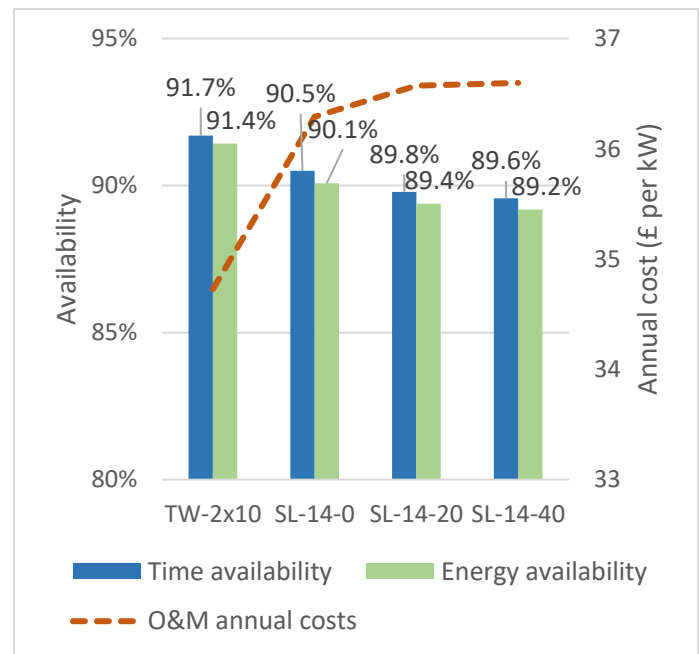
FIGURE 7. AVAILABILITY AND COST RESULTS OF THE SIMULATED SCENARIOS.
