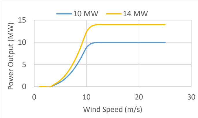
FIGURE 6. POWER CURVES FOR 10 MW AND 14 MW TURBINES.
