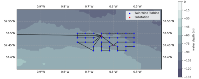
FIGURE 4. FLOATING WIND FARM LAYOUT WITH 35 TWIN 10MW TURBINES.
