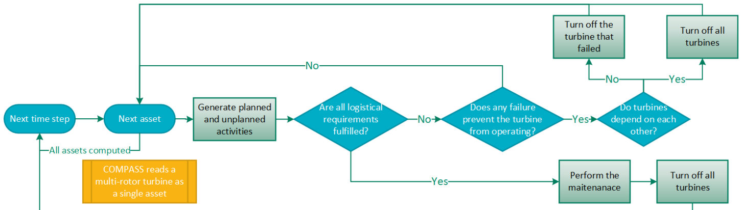
FIGURE 1. SIMPLIFIED FLOWCHART SHOWING THE SIMULATION LOGIC FOR TWIN TURBINE MAINTENANCE.
