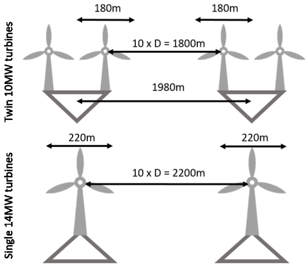
FIGURE 3. DISTANCES BETWEEN TURBINES AND FOUNDATIONS.
