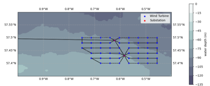
FIGURE 5. FLOATING WIND FARM LAYOUT WITH 50 SINGLE 14MW TURBINES.
