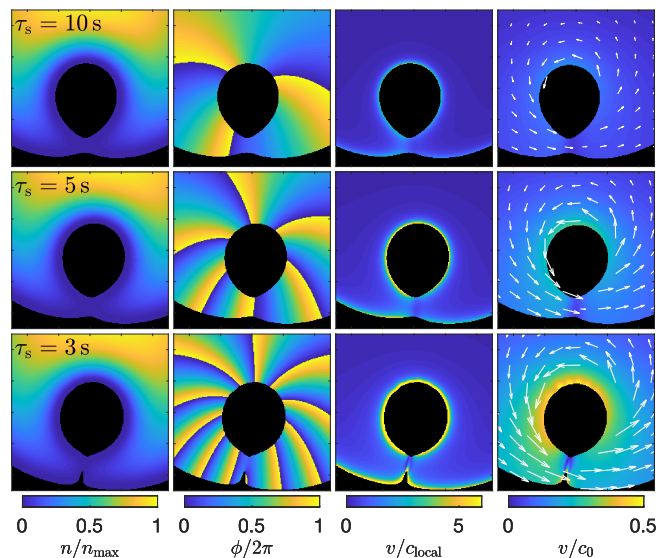
FIG. 5. Snapshots from 2D GPE simulations for varying \tau_s (as labeled). Snapshots show the timepoint t_m \sim 0.66\tau_s where the flow behind the beam merges with that ahead of the beam resulting in continuous superflow around the beam. Columns from left to right show zoomed in snapshots of (i) density, (ii) phase, (iii) the velocity profile scaled to the local speed of sound, and (iv) the velocity profile scaled to the bulk speed of sound c_0 (using the peak density n_0 ). White arrows indicate the direction of the flow. Simulation parameters are N_s = 4 , R_0 = R_r , w_0 = 18 \mu\text{m} , and U = \mu_0 . Note the dark soliton appearing in the reconnecting flow for \tau_s = 3 s.
