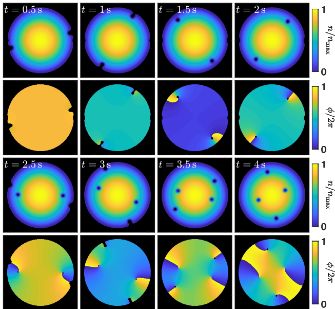
FIG. 10. GPE simulation for four beams. First one pair of beams spirals counter-clockwise. After 2 s of evolution, the second pair of beams begins to spiral clockwise. Simulation parameters are N_s = 4 , \tau_s = 5 s, w_0 = 4 \mu\text{m} , and U = \mu_0 .
