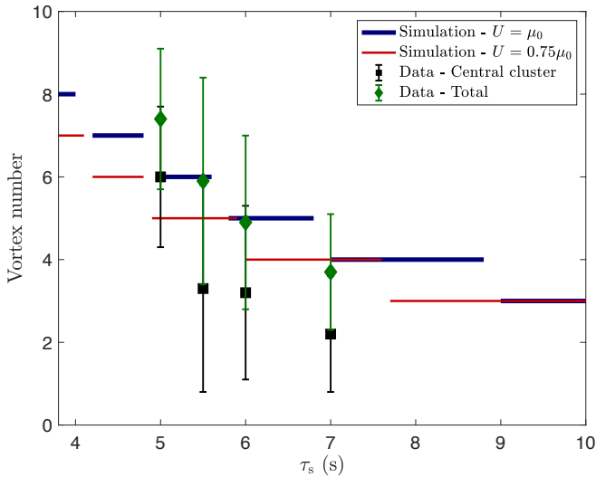
FIG. 7. Average number of vortices observed after ramping off the pinning potential as a function of trajectory duration \tau_s , for fixed N_s = 4 and beamwaist w_0 = 18 \mu\text{m} . Black squares and green diamonds correspond to experimental data, while solid blue and red lines are numerical results from the 2D GPE simulations. Black squares show the average number of cores in the central cluster, whereas green diamonds show the average total number of vortex cores. Error bars indicate the standard deviation. Solid blue lines correspond to a spiraling potential U = \mu_0 , and solid red lines correspond to U = 0.75\mu_0 . Both experiment and numerics show that the number of vortices generated and pinned using our method decreases as the optical potential moves more slowly through the condensate.
