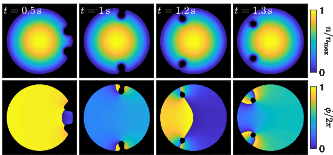
FIG. 9. GPE simulation for two beams, one spiraling clockwise and one spiraling counter-clockwise. Simulation parameters are N_s = 2 , \tau_s = 3 s, w_0 = 8 \mu\text{m} , and U = \mu_0 .
