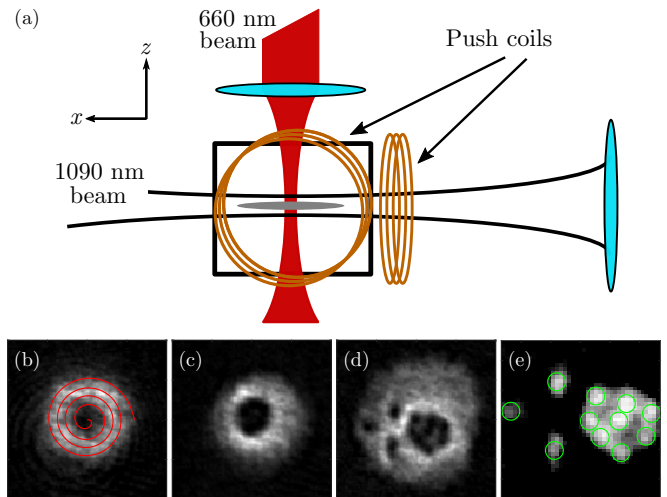
FIG. 2. Experimental setup. (a) Schematic of the experimental setup (not to scale). (b)-(d) Axial absorption images showing a 200\text{-}\mu\text{m} square field of view in the horizontal x - y plane. (b) In-trap image of the BEC with the 660-nm blue-detuned beam at its center. Also shown is the effective spiral trajectory [red line] of the 660-nm beam as the condensate is translated by time-varying magnetic fields. (c) BEC after ballistic expansion. The BEC is allowed to expand right after the pinning optical potential is ramped off ( t_d = 0 ms, see text). The large hole in the center of the condensate is taken as evidence of multiply-charged superflow since its size is much larger than a single vortex core. (d) BEC with 11 singly-quantized vortices, imaged after ballistic expansion. Here we wait for t_d = 160 ms between the 660-nm beam ramp off and ballistic expansion to allow the superflow to disperse into singly-quantized vortices. (e) Residuals from Thomas-Fermi fit to the image shown in (d), zoomed in to the central vortex region. Green circles indicate individual vortex cores.
