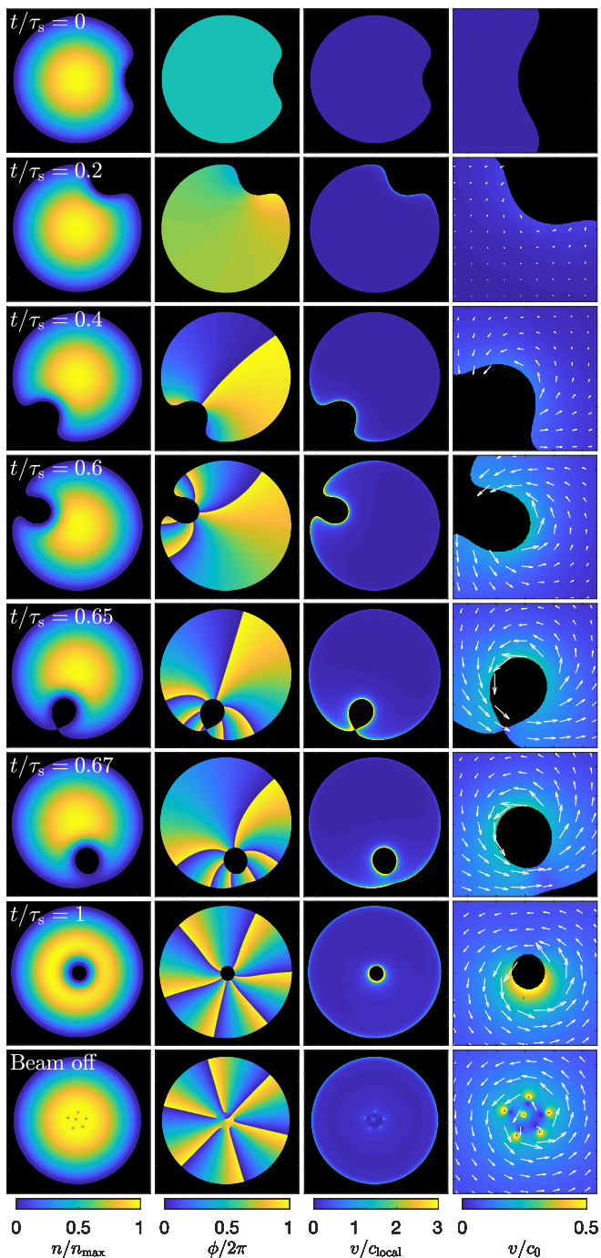
FIG. 4. Snapshots from 2D GPE simulation of the spiral technique at representative times t/\tau_s . Columns from left to right show snapshots of (i) density, (ii) phase, (iii) the velocity profile scaled to the local speed of sound, and (iv) a zoomed in region of the velocity profile at the location of the stirring beam. The velocity profile in column (iv) is scaled to the bulk speed of sound c_0 (using the peak density n_0 ). White arrows indicate the direction of the flow. Simulation parameters are N_s = 4 , \tau_s = 5 s, R_0 = R_r , w_0 = 18 \mu\text{m} , and U = \mu_0 .
