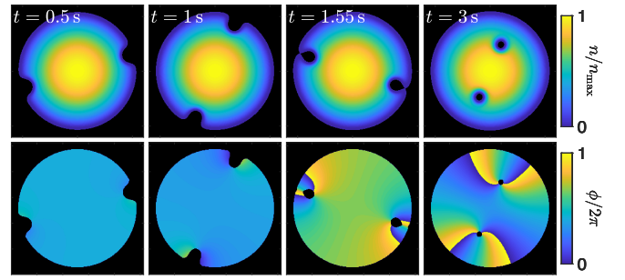
FIG. 8. GPE simulation for two beams both spiraling counter-clockwise. Simulation parameters are N_s = 3 , \tau_s = 4 s, w_0 = 8 \mu\text{m} , and U = \mu_0 .
