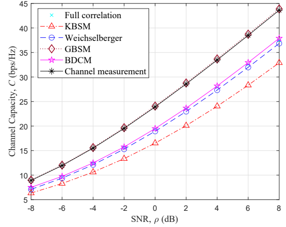
Fig. 8. Channel capacities of various channel models.
