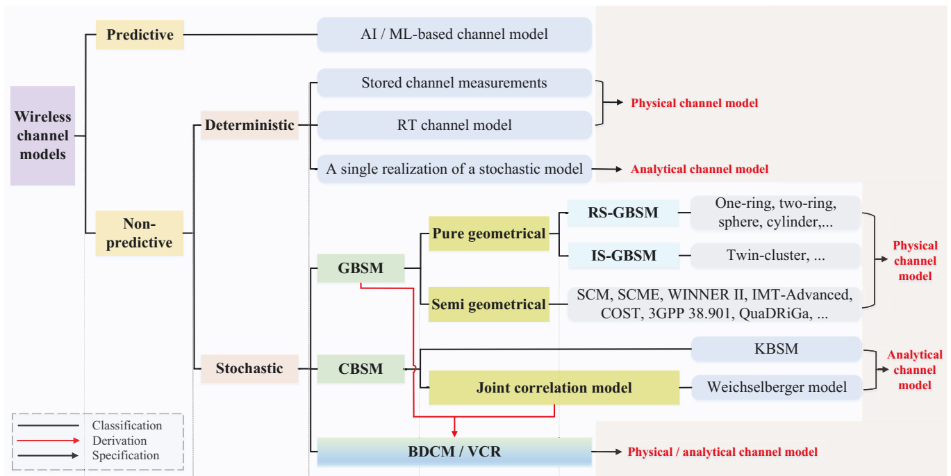
Fig. 4. A proposed classification method of wireless channel models.
