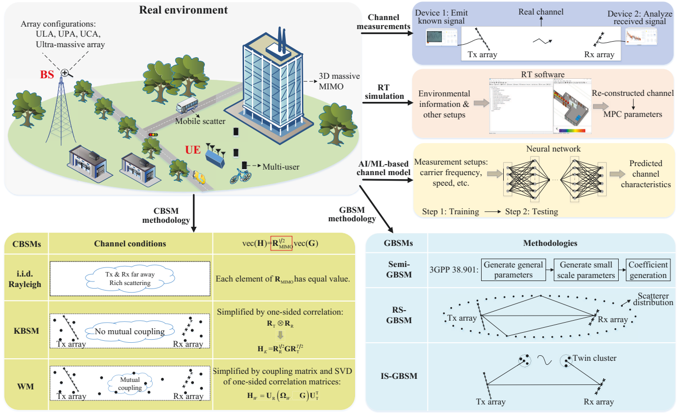
Fig. 5. Massive MIMO communication environment and abstracted channel models.
