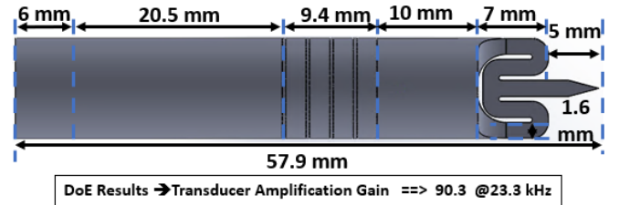
Figure 6. The optimised PF transducer.
