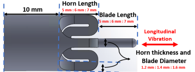
Figure 4. The investigated parameters for twice planar folded front mass. A. Stack material, placement, vibration amplitude considerations
