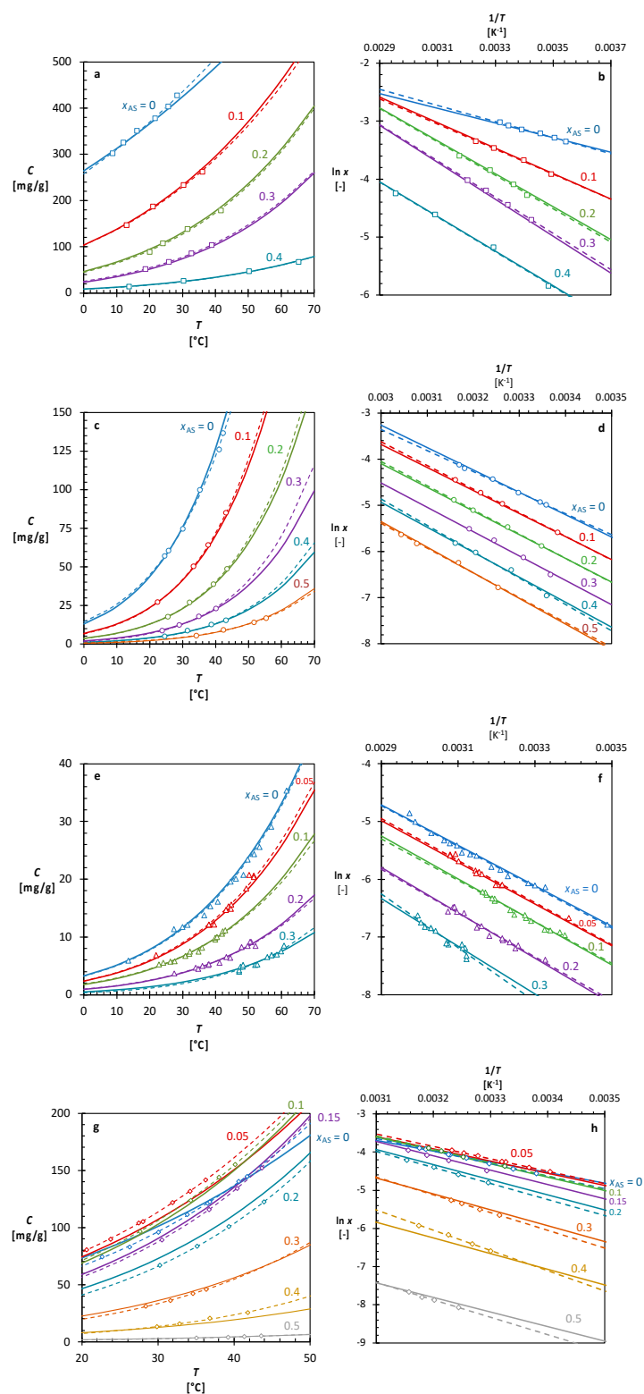
Figure 4. Concentration–temperature (left) and \ln x – 1/T (right) diagrams of: (a,b). ( \square ) \text{NaBrO}_3 in water–ethanol, (c,d). ( \circ ) ASN in water–ethanol, (e,f). ( \triangle ) MFA in ethanol/water, and (g,h). ( \diamond ) LOV in acetone/water at various antisolvent fractions. The experimental data are represented by the markers, with the colours and labels representing the antisolvent fraction. The dashed lines give the best fit of the data at a specific antisolvent fraction to Equation (2). The solid lines represent the predicted solubility at each antisolvent fraction using the best fit of all data to Equation (4).
