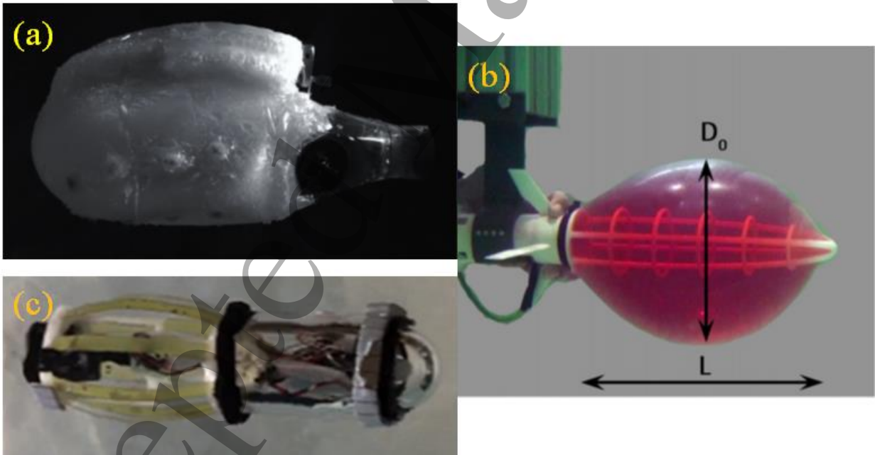
Figure 6. Examples of existing designs of deformable swimmers inspired by squids: (a) an elastic swimmer driven by motor and cables (reproduced from [61] with permission of IOP Science), (b) an ultra-fast swimmer driven by elastic energy stored in its skin (reproduced from [77] with permission of IOP Science), and (c) a deformable swimmer with elastic skin and ribs driven by motor with a slip-gear design (reproduced from [60] with permission of IOP Science).
