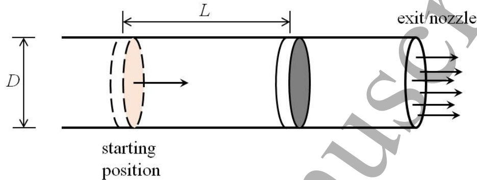
Figure 4. Definition of the stroke ratio L/D based on the piston-cylinder setup.
