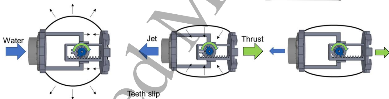
Figure 7. A hybrid activation system including a DC motor, a slip-gear system, and elastic energy storing/release system with elastic skin and ribs. In this design the gear is engaged during inflation (the left figure) so that the body deformation is driven by the motor. During deflation (the other two figures) the gear detaches and the elastic energy in the system is released. This figure is reproduced from [60] with permission of IOP Science.
