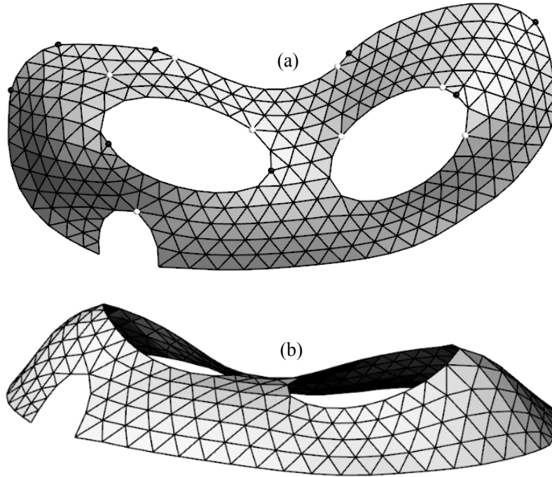
Fig.25 Grid by the connectivity regularization and net-like method: (a) Top view and (b) Perspective view
