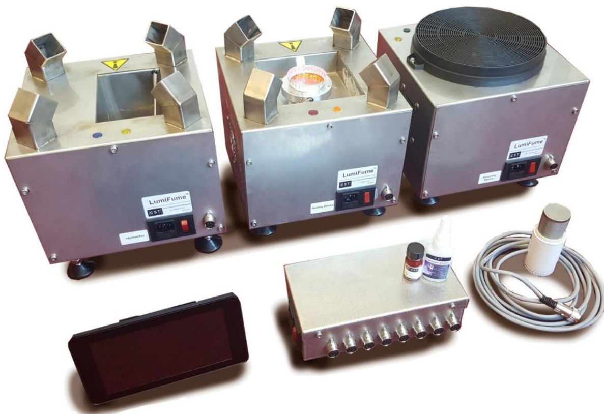
Figure 2 – The LumiFume™ crime scene cyanoacrylate fuming system [31].
