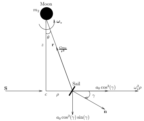
Figure 3. Representative forces.
