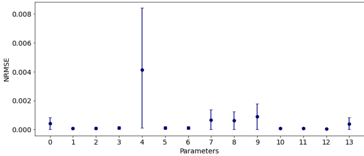
Fig. 6. Average NRMSE with CI 95% of the analysed parameters with injected anomalies in parameter 4.
