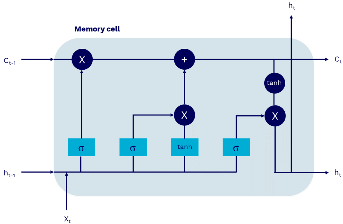
Fig. 3. LSTM cell architecture.
