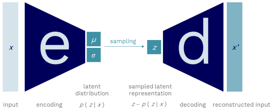
Fig. 2. VAE architecture.
