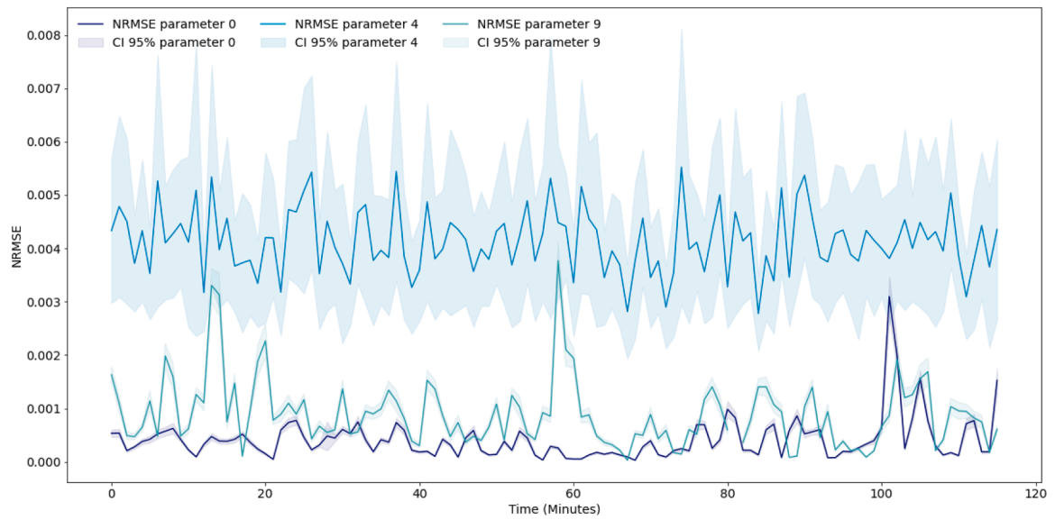
Fig. 7. NRMSE with CI 95% of parameters 0, 4, and 9 divided by instance with injected anomalies in parameter 4.
