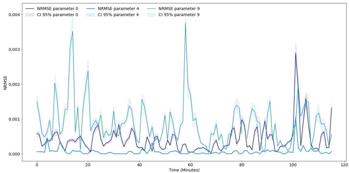
Fig. 9. NRMSE with CI 95% of parameters 0, 4, and 9 divided by instance.
