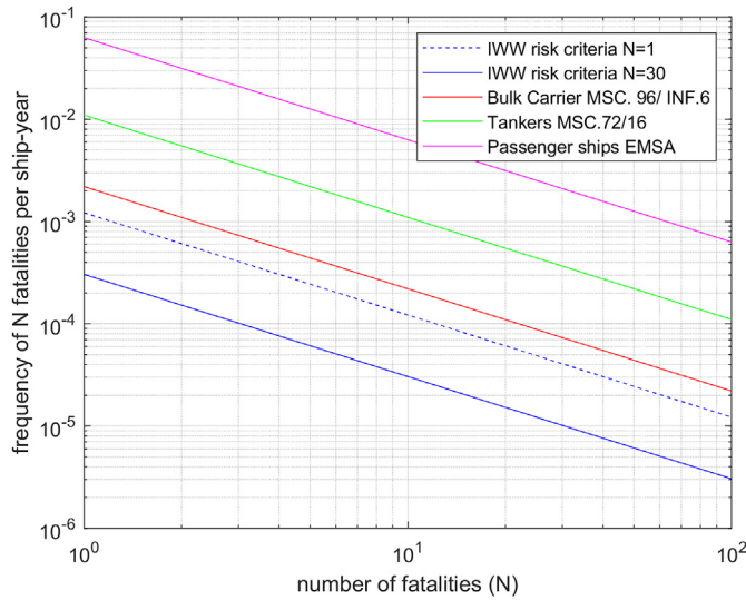
Fig. 2. Societal risk acceptable level (only the border between tolerable and intolerable levels are depicted).
