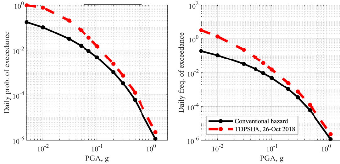
Figure 8. Short-term PSHA for Patras, left-hand panel: the short-term time-dependent daily probability of exceedance versus PGA and comparison with the conventional daily hazard curve and right-hand panel: short-term time-dependent daily rate of exceedance versus PGA and comparison with the conventional daily hazard curve.
