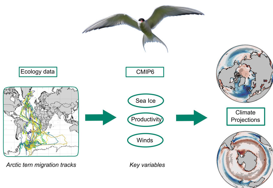
Figure 3. A schematic figure demonstrating the interdisciplinary approach to investigate the potential impacts of climate change on Arctic terns ( Sterna paradisaea ), a small seabird that annually undertakes the longest recorded migration. CMIP6 models were used to predict changes to key environmental variables that are likely to affect this species during their transequatorial migration and non-breeding periods in the Southern Ocean during the austral summer.
