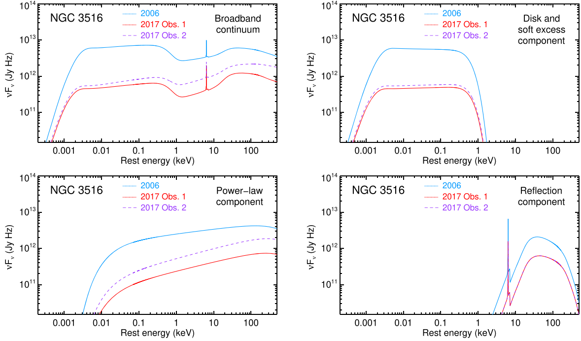
Figure 4. Derived intrinsic broadband SED model for the high-flux state (2006) and the low-flux state (2017) of NGC 3516. The total broadband continuum model is shown in the top left panel. The individual components of the SED model are displayed in the other panels: the disk and the soft X-ray excess component ( comt , top right panel), the X-ray power-law continuum component ( pow , bottom left panel), and the X-ray reflection component ( refl , bottom right panel). All continuum components of the SED have become fainter in the new changing-look state of NGC 3516 in 2017.
