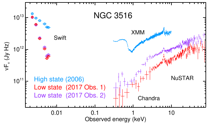
Figure 2. Optical/UV and X-ray spectra of NGC 3516 taken during the high-flux state in 2006 and the low-flux state in 2017. The data are from Chandra/LETG (2017), NuSTAR (2017), XMM-Newton/EPIC-pn (2006), and Swift/UVOT (2006 and 2017). The displayed data include the host galaxy emission and the effects of intrinsic and Galactic absorption and reddening. The displayed X-ray spectra have been binned for clarity of presentation. The best-fit model to these data is shown in Figure 3 and the derived intrinsic continuum model in Figure 4. Transformation in shape and flux of the multi-wavelength spectrum between the two epochs is evident.
