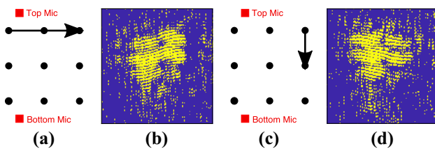
Fig. 6 Two strokes with different direction information. a A stroke that is moving away from the bottom microphone. b Connected components (CC) of the stroke shown in a extracted from the bottom microphone. It shows an ascending trend. c A stroke that is moving towards the bottom microphone. d CC of the stroke in c extracted from the bottom microphone. It shows a descending trend
