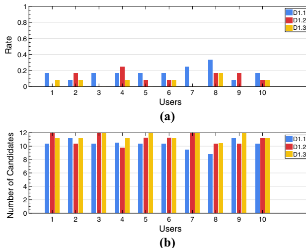
Fig. 12 Results per user with decision method D1. a Pattern guess rate (Metric M1). b Average number of pattern candidates remained after predictions (Metric M2)
