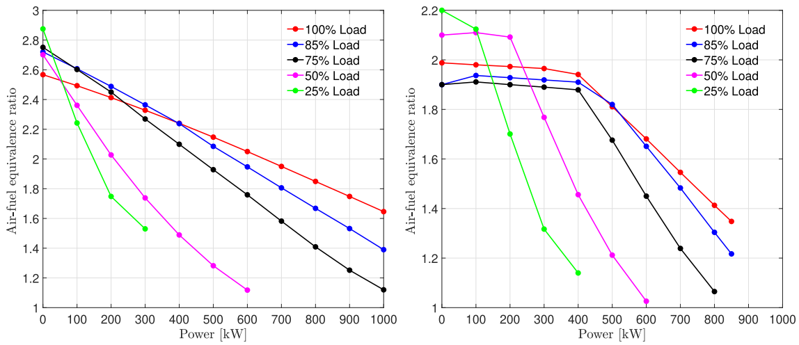
(a) Air-Fuel equivalence ratio-Diesel Mode. (b) Air-Fuel equivalence ratio-Gas Mode.
