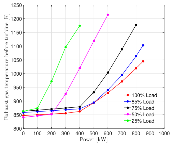
(f) Exhaust gas temperature before turbine–Gas Mode.
