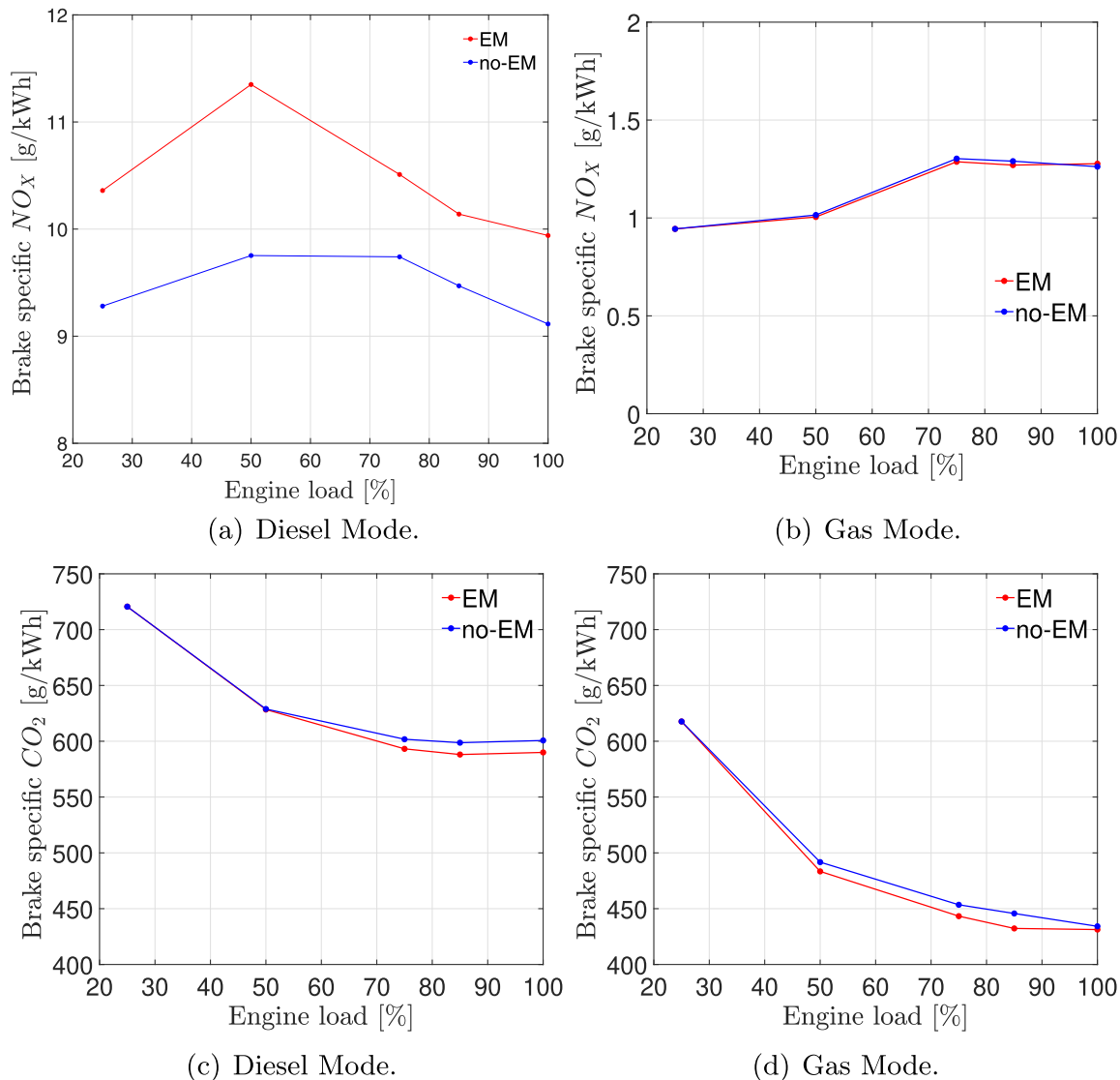
Fig. 9. Corrected Brake Specific NO_x and CO_2 emissions for the engine configurations with and without the selected HTC versus engine load at the diesel and gas operating modes.
