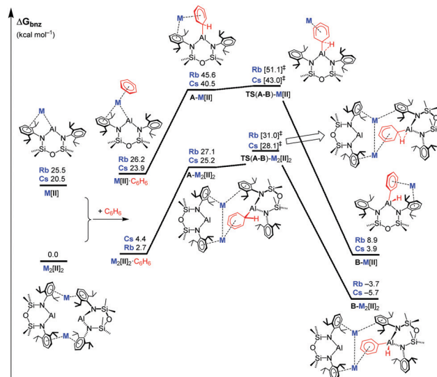
Fig. 3 DFT-calculated free energy profile (BP86-D3BJ/BS2(C 6 H 6 )/BP86/BS1) in kcal mol -1 for the C–H activation of benzene relative to 1 ( M = Rb ) or 2 ( M = Cs ). See Fig. S25 (ESI†) for a larger version.
