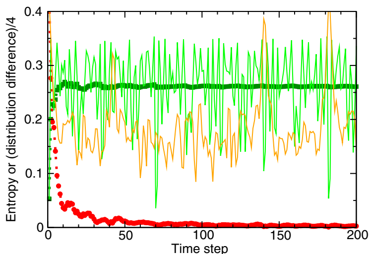
Figure 13. Comparison of time-averaged entropy (thick green) with convergence to time-averaged limiting (uniform in this case) distribution (thick red) for a seven-cycle with symmetric initial coin state and Hadamard coin operator. The difference between the time-averaged distribution and the limiting distribution is scaled by a factor of 0.25 to make the range of fluctuations roughly comparable with the entropy, and shown by the instantaneous entropy and distribution difference (thin lines).
