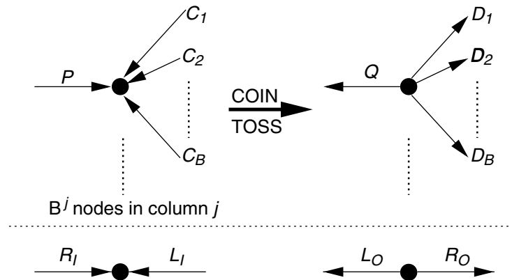
Figure 20. Typical node in the left-hand tree before and after the coin operator is applied, showing our notation for mapping the walk to a line. P, Q, \{C_i\}, \{D_i\}, R_l, R_o, L_l, L_o are amplitudes.
