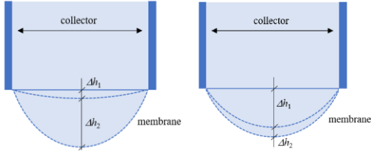
Figure 2 Deformation under static pressure with (a) hyper-elastic model (b) linear-elastic model
