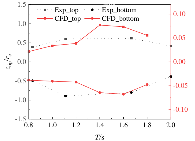
Figure 9 Maximum and minimum tip displacement with T=0.8s-2.0s
