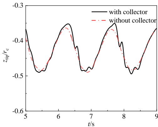
Figure 8 Tip displacement for a flexible WEC
