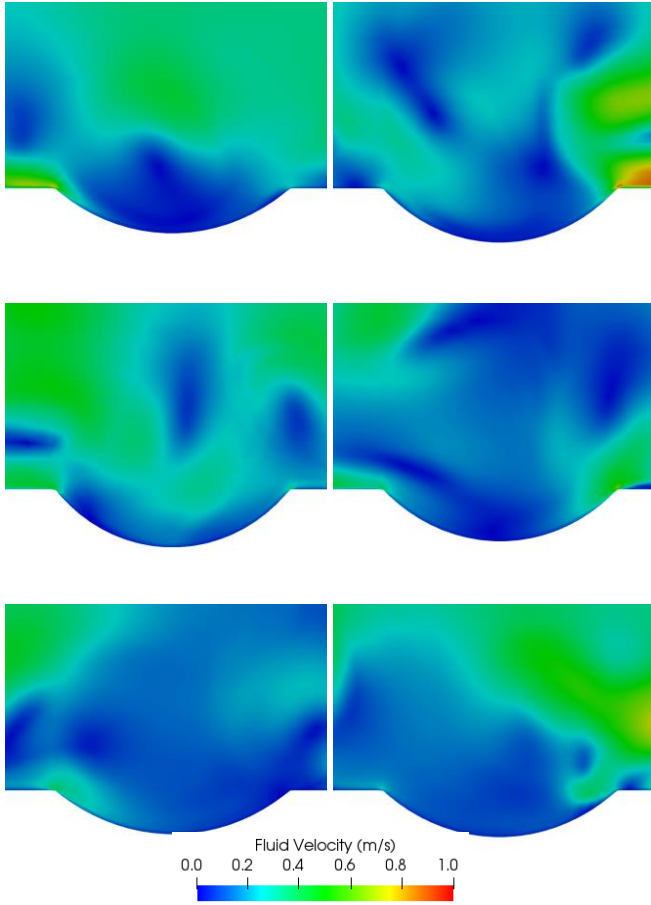
Figure 8 Velocity field around the collector from t=5.1s to t=6.6s
