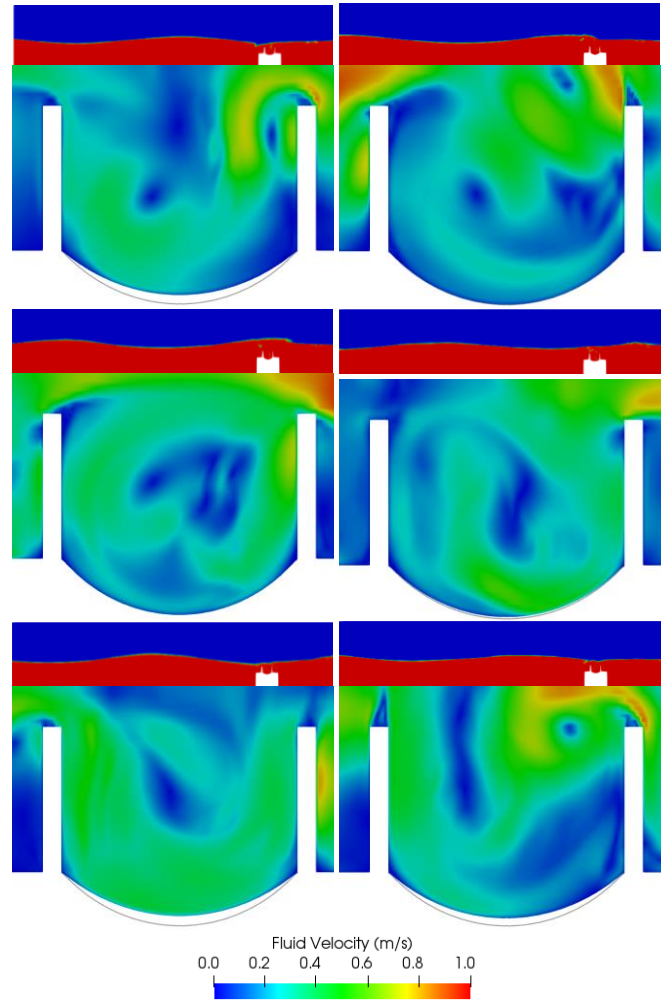
Figure 6 Free surface in the wave tank and velocity field around the collector from t_7=5.1s to t_{12}=6.6s . upper image is the volume fraction field in the whole tank. The lower image is the zoomed-in velocity field around the collector. The solid curve below the membrane is the maximum deformation position for comparison.
