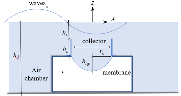
Figure 1 Sketch of a flexible WEC model
