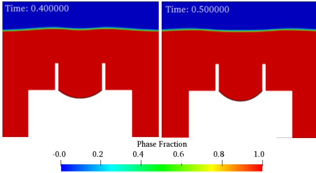
Figure 4 Free surface above the membrane from t_1=0s to t_6=0.5s . The blue and red areas represent air and water
