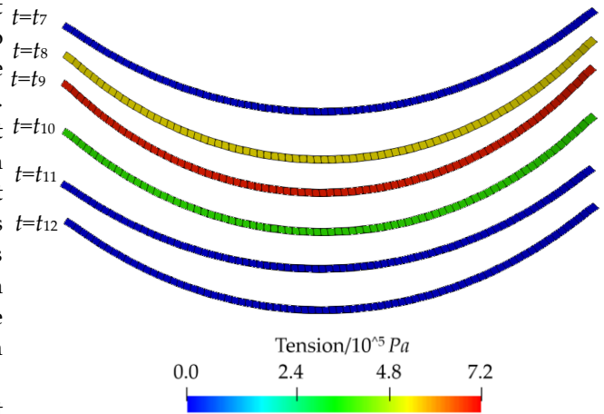
Figure 7 Shape and tension of the membrane from t_7=5.1s to t_{12}=6.6
