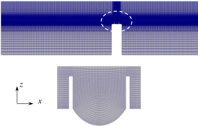
Figure 3 CFD mesh (a) of whole wave tank (b) around the membrane
