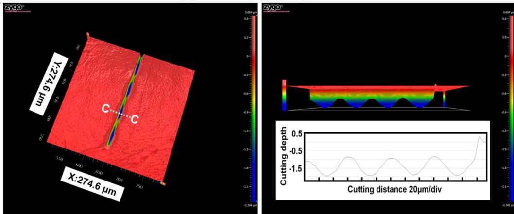
(c) T=20s , v=3 \mu\text{m/s}
