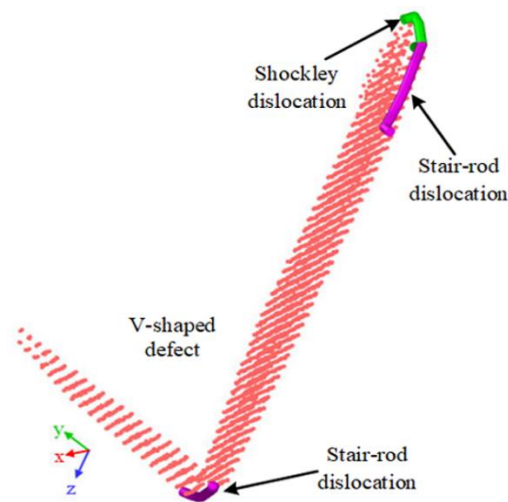
Fig. 12. Atomic snapshot of V-shaped defect.
