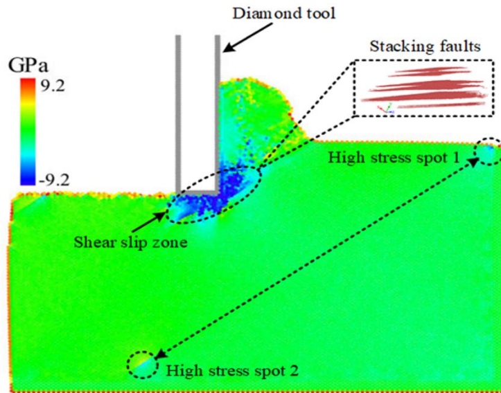
Fig. 15. Hydrostatic stress distribution of cutting zone of single crystal copper.
