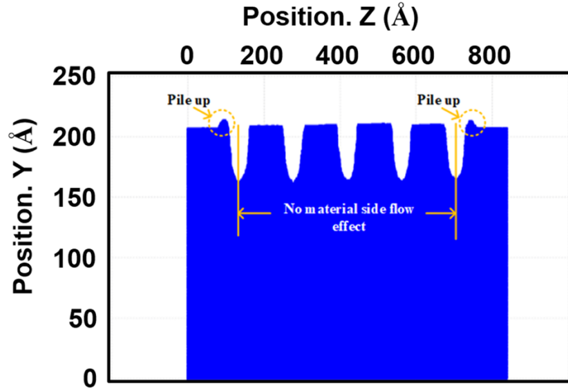
Fig. 10. Cross-sectional of machined periodic nanogrooves from MD simulation results.
