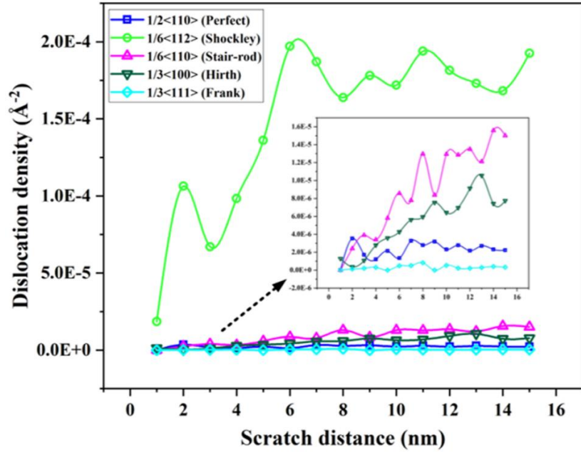
Fig. 14. Variation of density of five types of dislocations.
