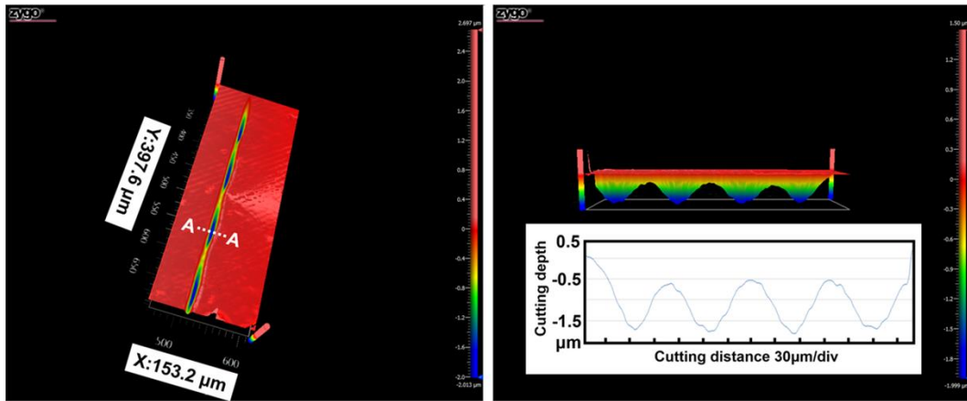
(a) T=5s , v=20 \mu\text{m/s}
