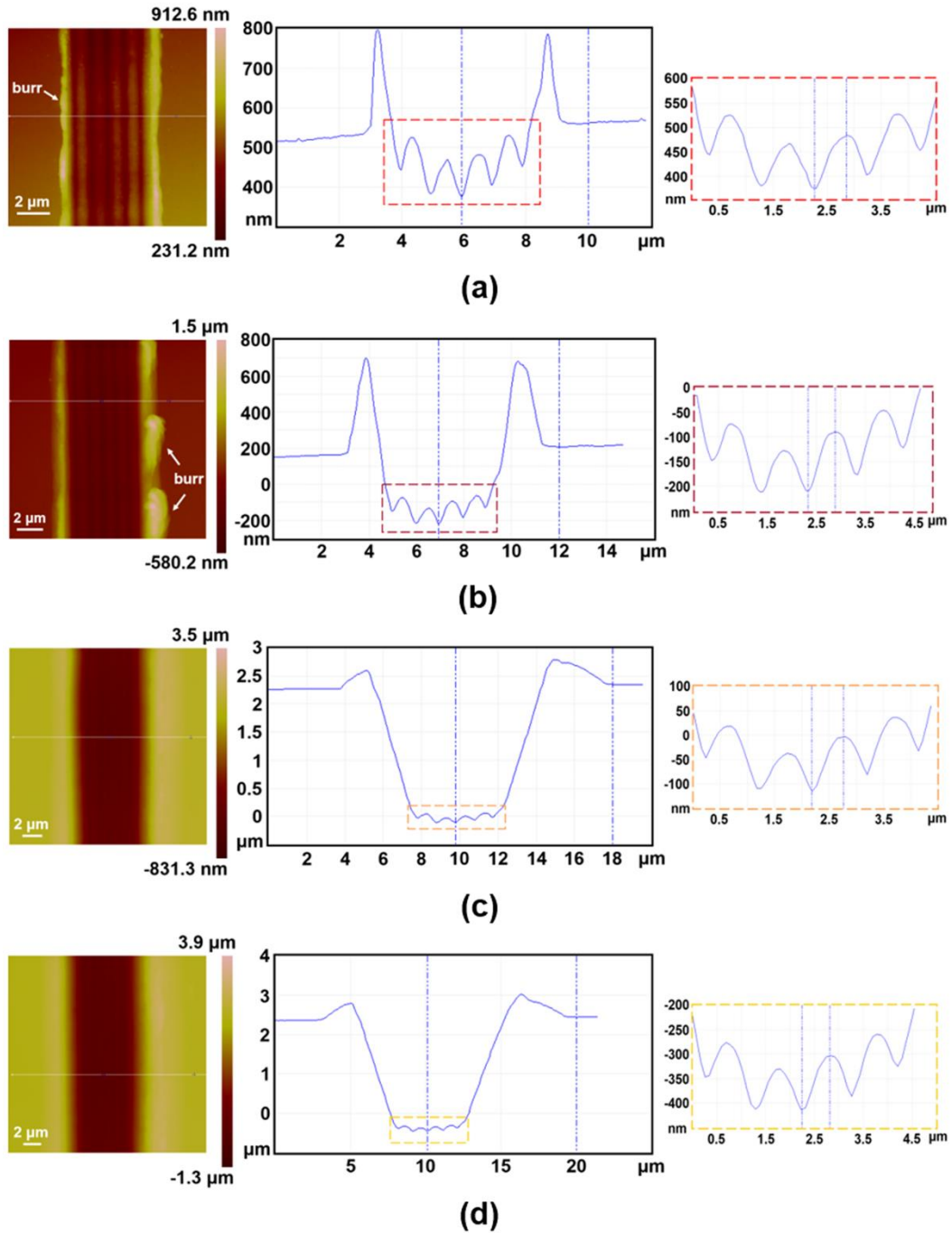
Fig. 5. AFM images of periodic sinusoidal microgrooves machined on the flat copper surface corresponding to the cutting forces: (a) 5 mN, (b) 10 mN, (c) 12 mN and (d) 17 mN.
