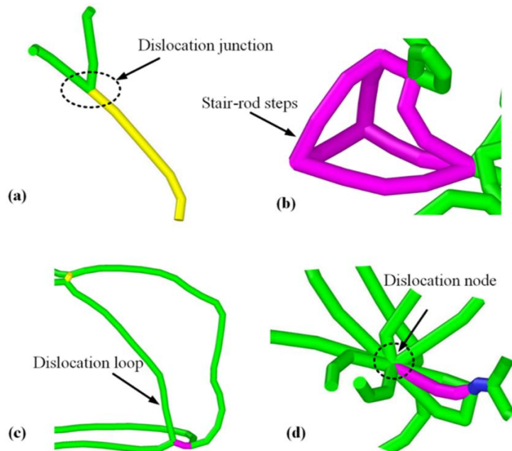
Fig. 13. Evolution of dislocations in the sub-surface of single crystal copper during MTD tool nanoscratching.
