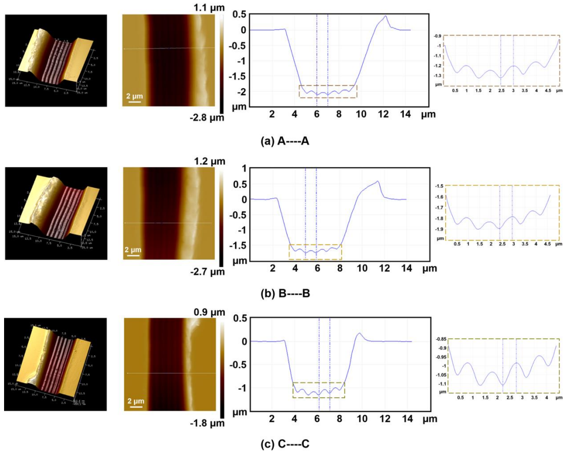
Fig. 9. Cross-sectional images of the machined ripples corresponding to figure 8.
