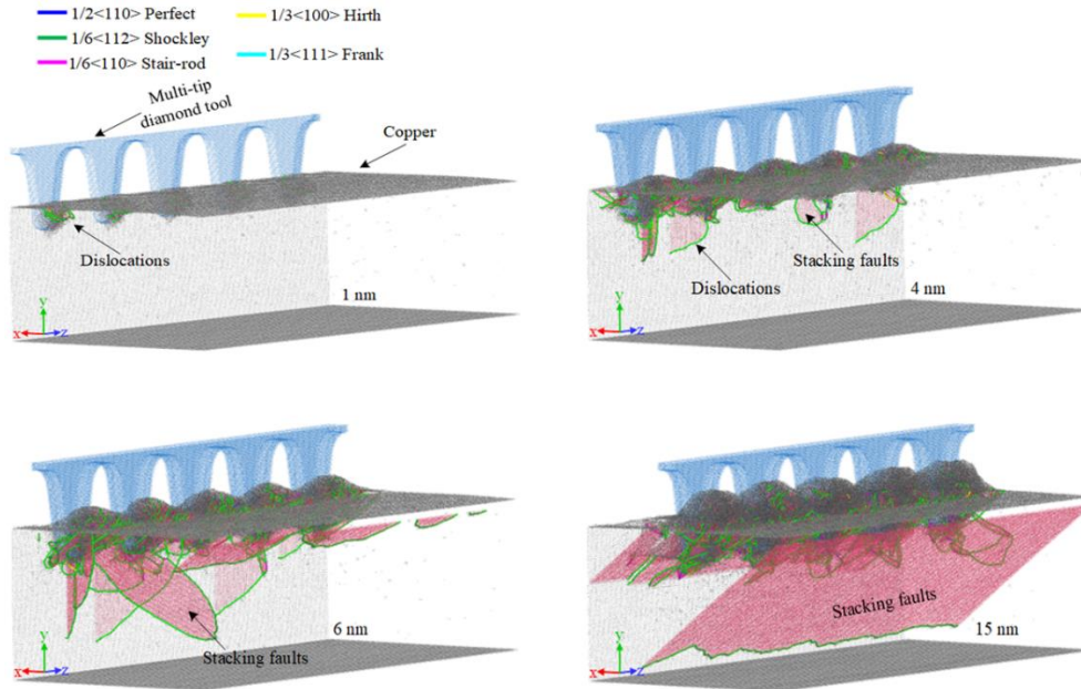
Fig. 11. Atomic snapshots of dislocations and stacking faults at scratching distance of 1 nm, 4 nm, 6 nm and 15 nm.
