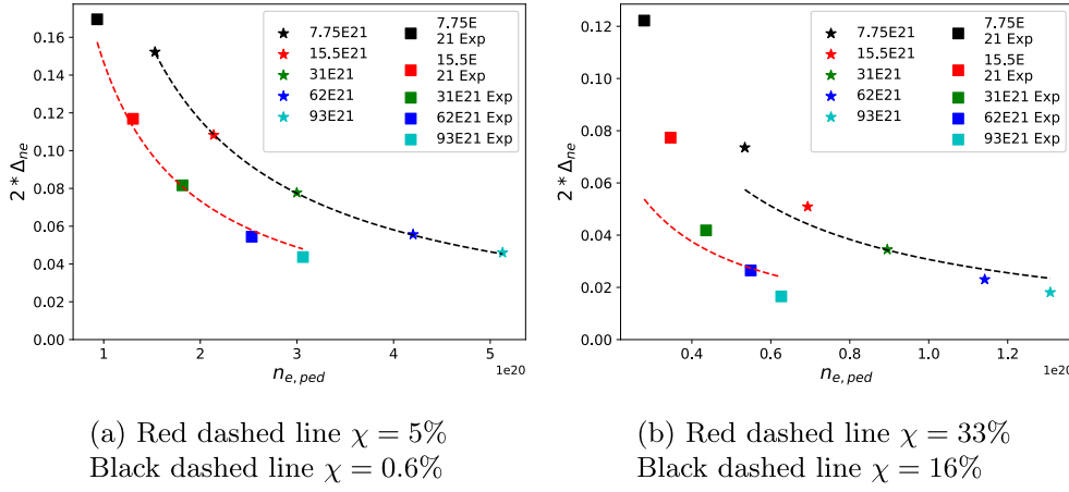
Fig. 4. A neutral source scan where the neutral source is placed either at the (a) outer midplane or (b) X-point. \Delta_{ne} , and n_{e,ped} , are calculated from fitting Eq. (6) to the predicted density profiles from JETTO-EIRENE. The x-axis for fit is taken to be the coordinate at the OMP (red line in Fig. 1a). The stars represent a simulation set up with a constant temperature profile and charge exchange (CX) turned off and the squares using the experimental T_e and T_i profiles and CX turned on. The dashed lines are the 1/n_{e,ped} , fits to \Delta_{ne} , and n_{e,ped} , of each data set (stars or squares). The neutral source scan shown here ranges from 7.75 \times 10^{21} to 93 \times 10^{21} atoms per second denoted by changing colour as shown on the legend of the figure.
