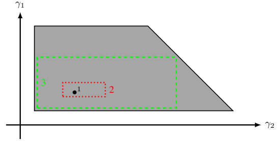
Figure 2: A graphical representation of IRR: starting from the parameter values from the original plan (depicted as the black point), IRR tries to construct increasingly better under-approximations (the colored rectangles) of the RE (the gray area), without actually computing it. Upon termination, each edge of the resulting DRE is guaranteed to be at most \beta apart from the border of the actual region.
