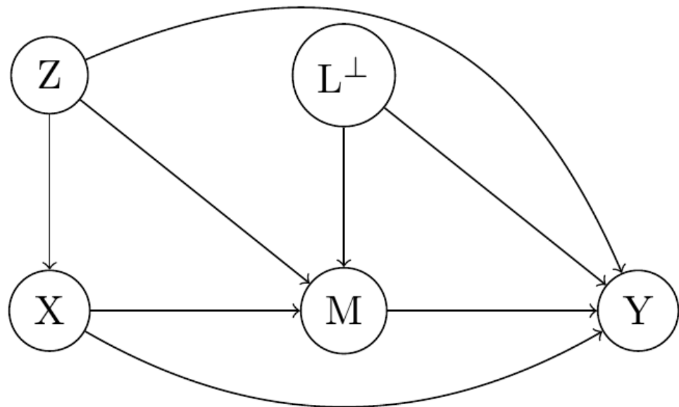
Figure 3: Causal relations between grandparent education ( X ), parental characteristics ( M ), and child cognitive ability ( Y ) in the presence of residualized post-treatment mediator–outcome confounders ( L^\perp ).
