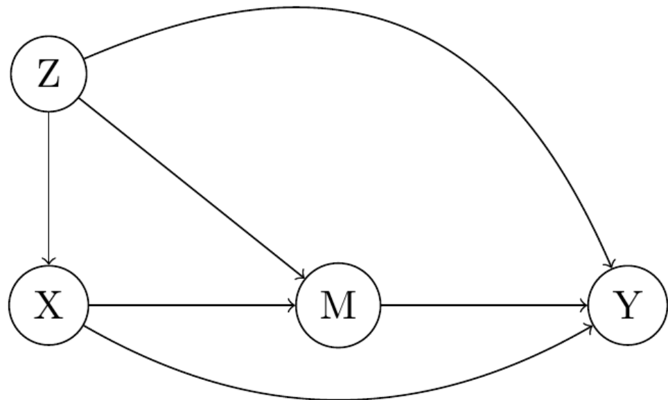
Figure 1: Causal relations between grandparent education (X), parental characteristics (M), and child cognitive ability (Y).
