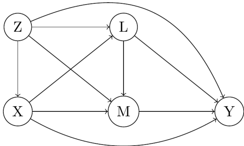
Figure 2: Causal relations between grandparent education (X), parental characteristics (M), and child cognitive ability (Y) in the presence of treatment-induced mediator–outcome confounders (L).
