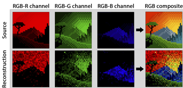
FIG. 7. Comparison between the source (upper row) and reconstructed (lower row) images for the individual color channels R/G/B (left plots) and the composite, full color RGB image (right plots). The contrast of the individual reconstructed channels and directly reconstructed composite image was adjusted to better match to the source images and allow for a clearer comparison.
