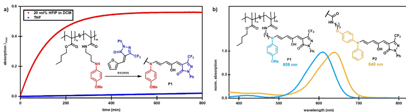
Figure 8. HFIP-promoted synthesis of DASA–polymer conjugates and properties of the resulting polymers. a) In situ absorption monitoring at \lambda_{\text{max}} (open form DASA) of the furan ring-opening reaction to afford P1 in THF or using HFIP in dichloromethane. b) Absorption spectra (chloroform) and chemical structures of DASA-functionalized poly(butyl methacrylate) polymers P1 and P2 ( m : 4 mol%).
