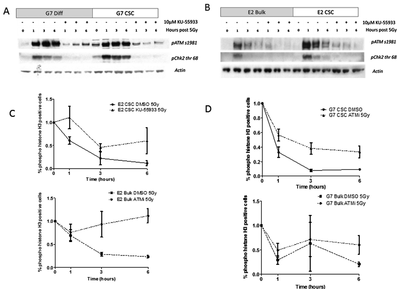
Figure 3 – Effect of KU-55933 on ATM and Chk2 phosphorylation and the G2/M checkpoint following ionising radiation. Extensions of the Western blots previously shown in Figure 2A are shown in A . G7 and B . E2, CSC and differentiated tumour cell cultures treated with 10 \mu M KU-55933 for 1 h prior to irradiation (5 Gy) and lysed at the time points shown following irradiation. Interrogation of the G2/M checkpoint by FACS analysis of mitotic cells identified by positive immunostaining of phosphorylated Histone H3 following treatment with 10 \mu M KU-55933 for 1 h prior to irradiation with 5 Gy in the C . E2 and D . G7 CSC and differentiated tumour cell cultures. Data points represent mean and SEM of 3 independent experiments.
