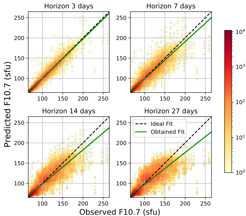
Fig. 8: Occurrence map of N-BEATS predicted values of the F10.7 with observed values over different forecast horizons for 2005-2020. The black dashed line represents the ideal R = 1 correlation, and the green line the fit obtained through linear regression.
