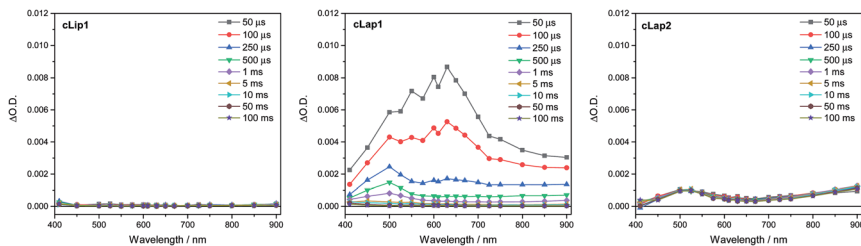
Fig. 5 \mu s to ms TA spectra (same scale on all y-axes) of cLiP1, cLaP1 and cLaP2 suspended in a H 2 O/TEA/MeOH mixture following excitation with a 355 nm laser (6 ns, 400 \mu J cm -2 , 0.33 Hz). The large TA features seen with cLaP1 correlate with the high rate of H 2 evolution.
