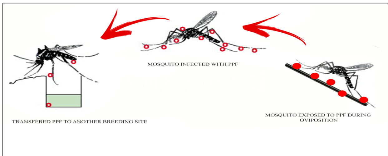
Figure 1. The mechanism of autodissemination of pyriproxyfen by female mosquitoes from exposure containers to other breeding sites.
