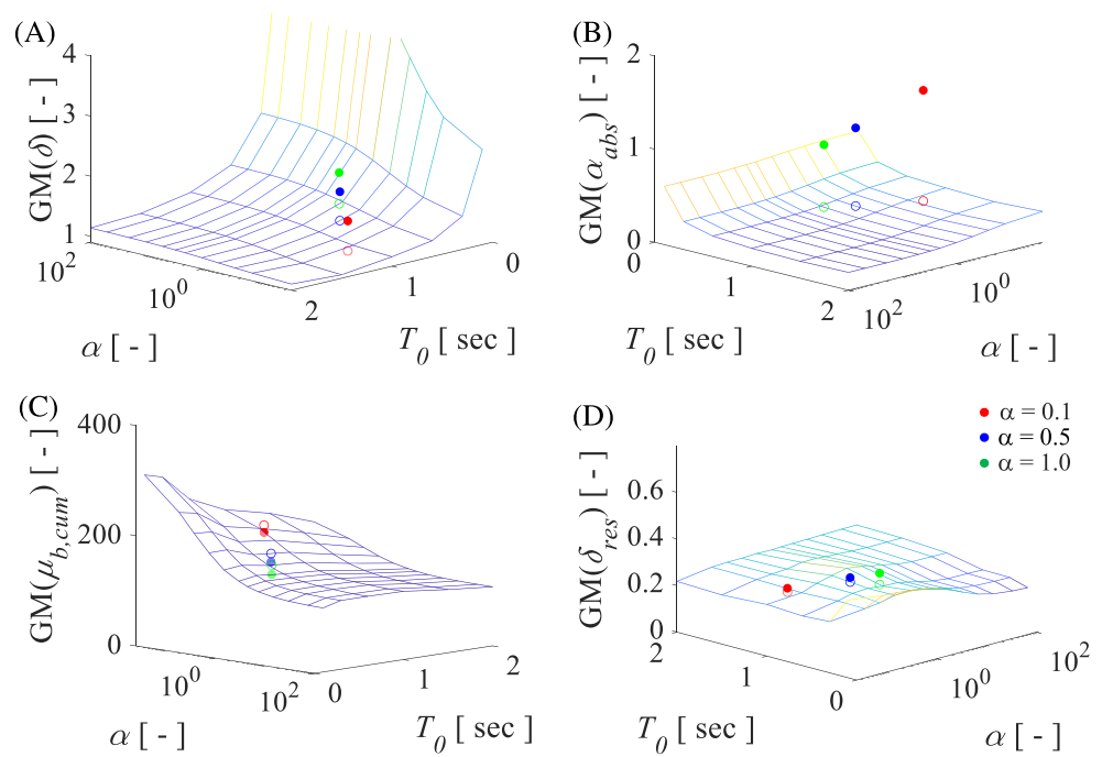
FIGURE 21 Seismic retrofitting of a RC MRF with BRBs. Comparison of the parametric analyses for SDOF and MDOF. Geometric mean (GM) of the A, normalized peak displacement demand \delta , B, normalized peak absolute accelerations demand \alpha_{abs} , C, BRBF's normalized cumulative ductility demand \mu_{b,cum} , D, normalized residual displacement demand \delta_{res} versus base shear ratio \alpha , for different values of T_0 and of \mu_{ft} = 4 and \mu_{bt} = 15 [Colour figure can be viewed at wileyonlinelibrary.com ]
