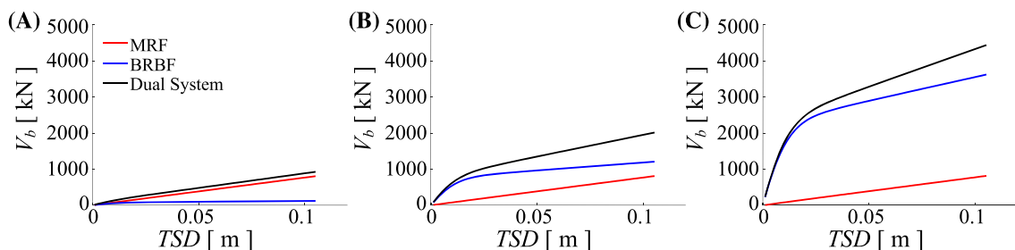
FIGURE 16 Newly designed dual steel MRF and BRBF. Pushover curves for \alpha equal to A, 0.1, B, 1, and C, 3 [Colour figure can be viewed at wileyonlinelibrary.com] [Colour figure can be viewed at wileyonlinelibrary.com]
