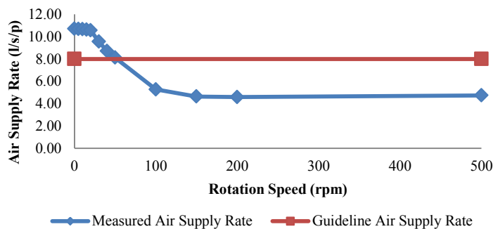
Figure 2. Measured air supply rates at increasing rotation speed of a rotary thermal wheel.
