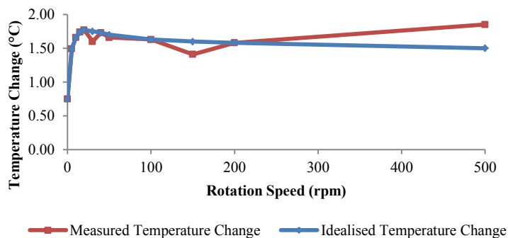
Figure 3. Temperature change of inlet macroclimate air passing through rotary thermal wheel as rotation speed increases
