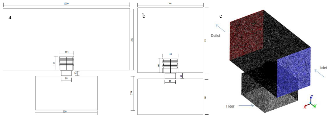
Figure 1. (a) Side view of geometry with dimensions; (b) end view of geometry with dimensions (dimensions in mm), (c) mesh generation of CFD domain
