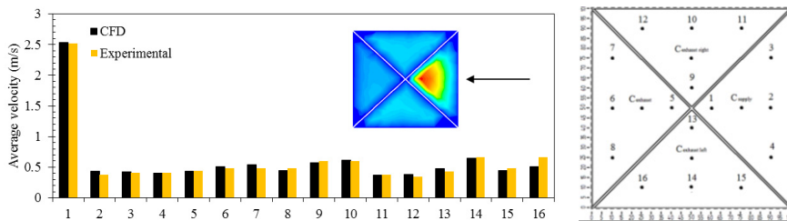
Fig. 6. Comparison between the experimental and CFD results of the airflow velocity measurement
