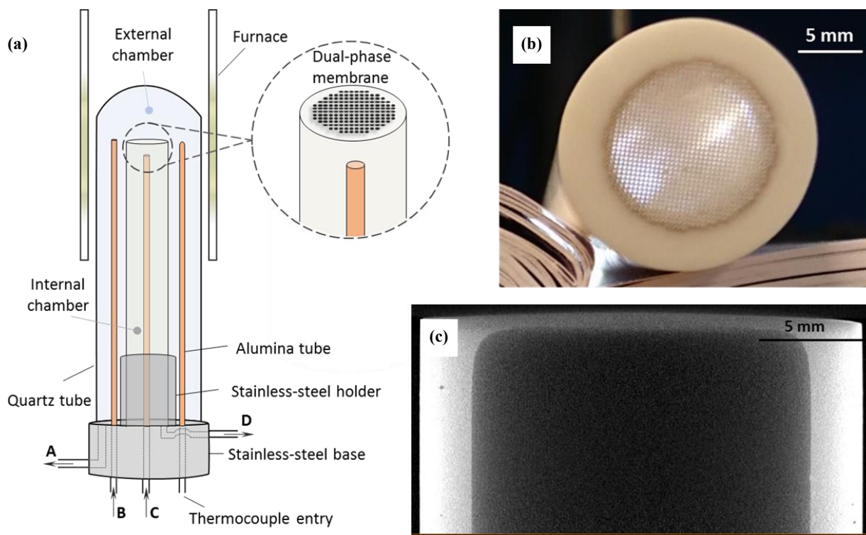
Figure. 4 Multiple-pore closed-end tube membrane and membrane reactor. (a) Multiple-pore membrane reactor, where A is the outlet of the feed-side chamber, with B the inlet, C is the inlet of the permeate-side chamber, with D the outlet. A thermocouple was positioned close to the membrane surface and the entire reactor placed within a furnace so that the stainless-steel base was outside the heating zone and a cold sealant could be used. (b) Digital image of the laser-drilled multiple-pore membrane. (c) X-ray micro-CT cross-section of the as-received closed-end tube.
