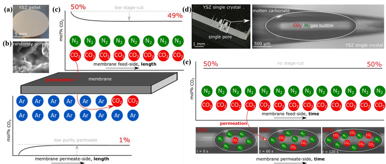
Figure. 1 Routine and visual permeation experiments. (a) Routine permeation measurements employ small pellet membranes ( \sim\text{cm}^2 ) with a, (b) randomly porous microstructure. (c) Such a membrane is operated with a low stage-cut and often an inert sweep gas (Ar) which imposes a large average driving force along the length of the membrane. Furthermore, the use of an inert sweep gas implies an infinite driving force at the sweep-gas inlet, and a low-purity permeate gas. Such conditions are not found in application. (d) Employing a single-crystal model membrane with a laser-drilled single pore allows the visualisation of an effect of permeation. Here, a \text{CO}_2/\text{N}_2 bubble occluded by molten carbonate inside the single pore is exposed to a flowing gas with a higher mole fraction of \text{CO}_2 . (e) Therefore, bubble volume increases with time and discrete driving forces can be accessed temporally. Note that during bubble growth, the permeate side of this
