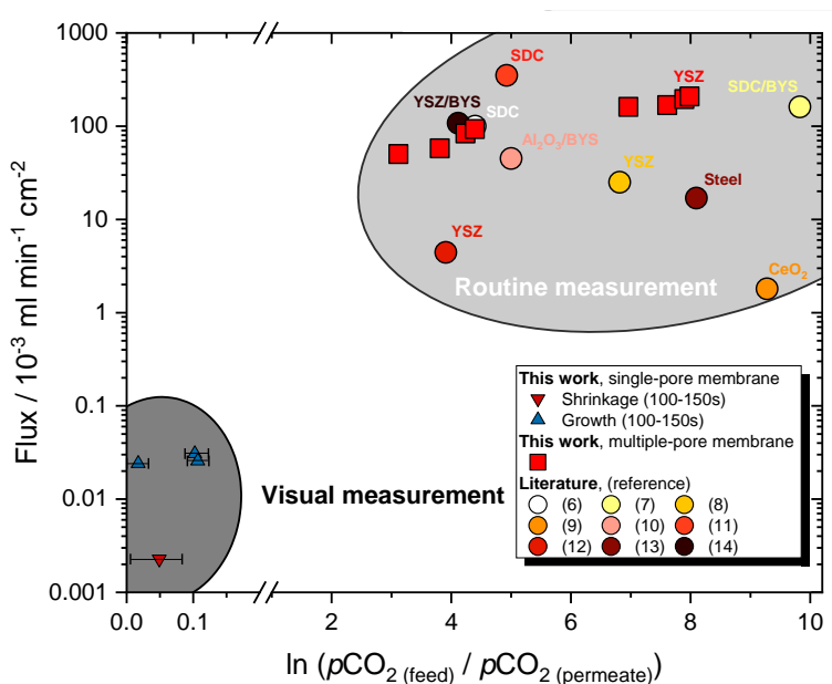
Figure. 3 Visual and routine flux measurements. Single-pore membranes and the visual method can probe a driving force region too challenging to access using routine measurements. Here, fluxes have been extracted from average permeation rates measured during 100 – 150 s in visual experiments (triangles and error bars, Supporting Information). The multiple-pore membrane accesses the routine measurement area but with a more well-defined membrane geometry. Representative data from the supported molten-salt membrane literature is provided (circles, with oxygen-ion conducting support material given). References in brackets can be referred to below.
