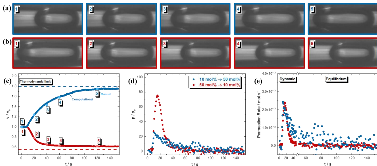
Figure. 2 Extraction of permeation rates from bubble volume changes. (a) Images of the growth of a 10 mol% CO 2 gas bubble following exposure to a flowing gas containing 50 mol% CO 2 and, (b) the reverse. (c) Normalised bubble volume variation calculated using manual image measurements at t = 0, 20, 40, 60 and 120 s (number labels correspond to images in (a) and (b)), and computational measurement of bubble volume with a temporal resolution of 0.255 s shown as a darker shade. The thermodynamic limit for bubble volume is shown as a dashed line (Supporting Information, Eq. S4 – S7). Detail on the manual and computational measurements is given in
