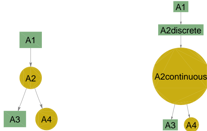
Figure 4: Graphical representation of the discretization procedure described
