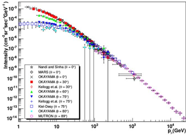
Figure 2. Muon intensity versus muon momentum, where \theta is the zenith angle [22].
