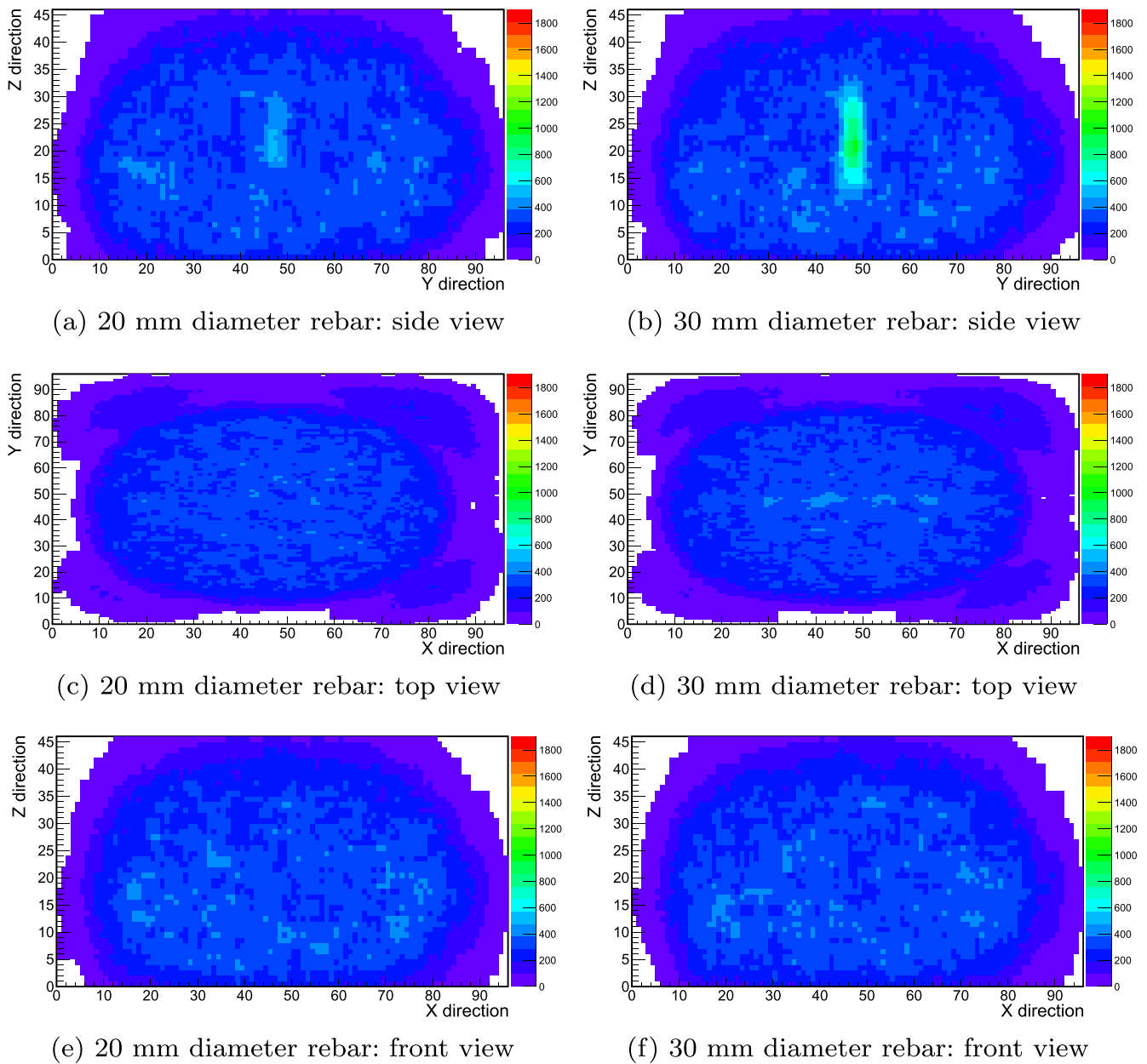
Figure 13. Images of the concrete object for the fixed size concrete blocks with rebars diameter of 20 (left) and 30 mm (right).
