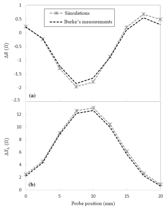
Fig. 7 Calculated values of the absolute coil's a resistance and, b inductive reactance as the coil scans over a notch. Comparison with impedance measurements extracted from Burke's work [28]
