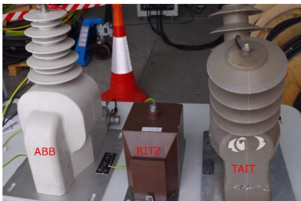
Figure 2: 11 kV voltage transformers used in testing at PNDC
