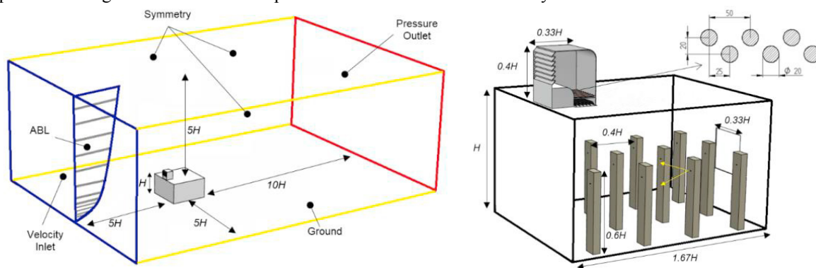
Fig. 2. (a) A roof mounted windcatcher with heat transfer devices (b) schematic diagram of the windcatcher operation.
