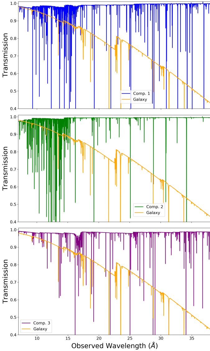
Fig. 3: Plot of PION absorption models for each warm absorber component (1 - 3 from top to bottom). These plots help demonstrate what the model looks like with the parameter values from Table 2: large \xi means absorption at higher energies; large N_H means stronger absorption lines. The Galaxy absorption transmission is overlaid in orange for a comparison. The Galaxy absorption affects the continuum emission, especially at longer wavelengths, causing the transmission to decrease. As a consequence of the RGS resolution, weak narrow lines are not evident in Figure 1 due to the low equivalent width, but can be seen in these models.
