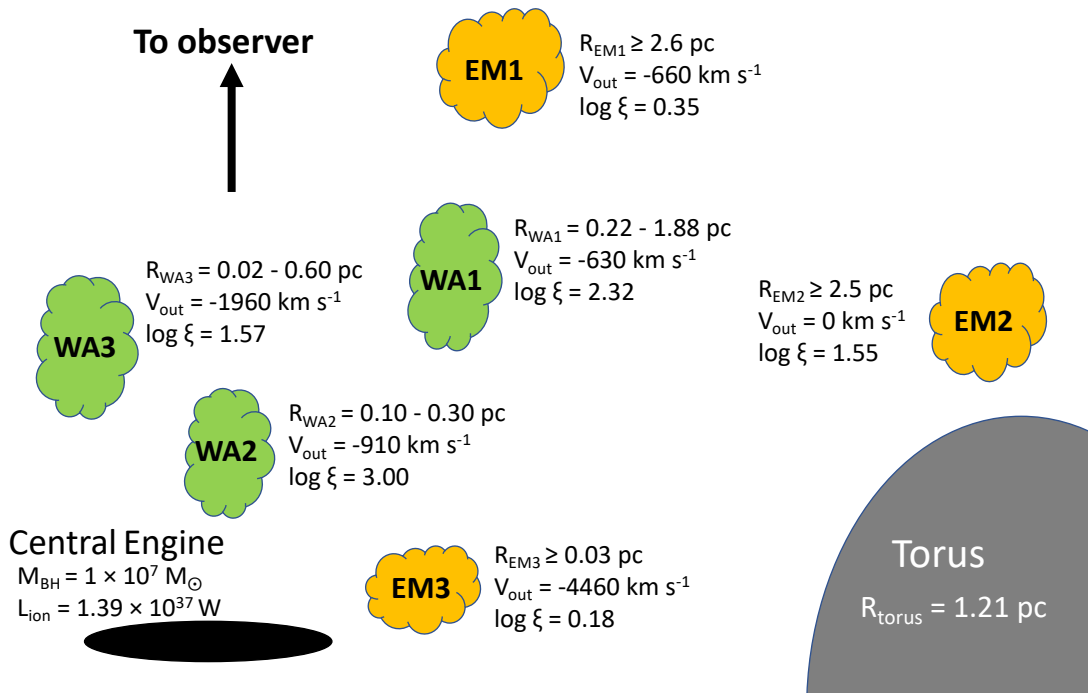
Fig. 7: Schematic display of the possible locations of the WAs (green) and emission line regions (orange) with respect to the central black hole. This graphic is not intended to show the exact locations of the photoionised plasma clouds, but can give insight into studying the physical scenarios. Next to each plasma cloud are the distances, ionisations and outflow velocities, depicted for an easy comparison. (The distances for the emission line regions are the lower limits, as obtained from Eq. 5.) As a comparison to the X-ray broad emission component (EM3), the optical BLR is at a distance of 0.004 pc in NGC 7469 (Kollatschny & Zetzl 2013).
