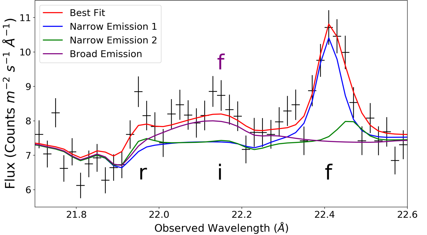
Fig. 5: Plot of the O VII He-like triplet in the observed frame of NGC 7469, with the three emission lines labelled in black (resonance, intercombination and forbidden for r, i and f, respectively). The spectrum (black crosses) is over imposed with the best fit model (red line). Two narrow components (EM1 and EM2) are shown by the blue and green lines, respectively, and a broad component (EM3) is plotted with the purple line. EM1 fits the forbidden line, EM2 fits the resonance line, as well as the forbidden line, and EM3 produces emission at location of the intercombination line, which is actually a broadened forbidden line with a large blueshifted velocity (as labelled with the purple ‘f’).
