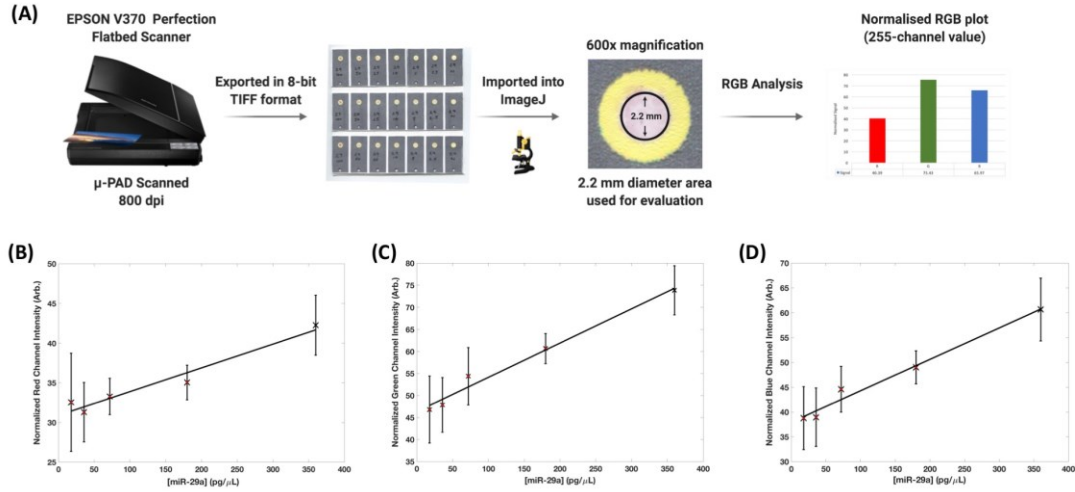
Figure 5. The protocol for RGB analysis is shown in A. After completion of the tests the paper-based devices were scanned using a flatbed scanner set at a resolution of 800 dpi. The exported 8-bit images were then uploaded into ImageJ. A circle of 2.2 mm diameter was used to define an area on all the test readouts and RGB analysis was carried out using the RGB measure script. Graphical representation of the colorimetric analysis of the 3D paper-based microfluidic devices. Each of the channels R, G and B are represented in that order from left to right (A-C). Each plot shows the relationship between normalized channel intensity and miR-29a concentration (18-360 pg/μL). Average values and standard deviations were generated from 3 replicates. Linear regression gave R^2 values of 0.9523 (red channel), 0.982 (green channel) and 0.9809 (blue channel). Red markers at lower miR-29a concentrations are used to highlight significant overlaps in the standard deviations.
