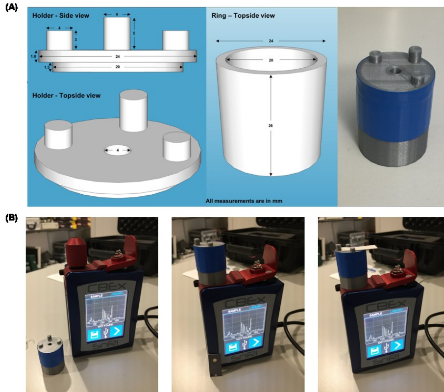
Figure 2. (A) shows the design and dimensions of the Raman aperture adaptor used for the analysis of the capture layer contained within the 3-D paper device. The adaptor was appropriately scaled to ensure that readouts were made at the optimal distance and center of the spot (B) Images display how the adaptor fits over the point and shoot lens and how the capture layer is mounted to enable SERS analysis.
