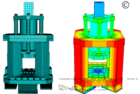
Fig. 1 Machine dynamics analysis with an FEM
