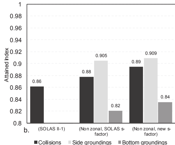
Figure 15: Comparison of survivability based on static calculations for: a.) Ship A b.) Ship C
