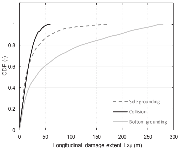
Figure 6: Cumulative distribution of the longitudinal damage extent (length) L_{x,p} for ship A
