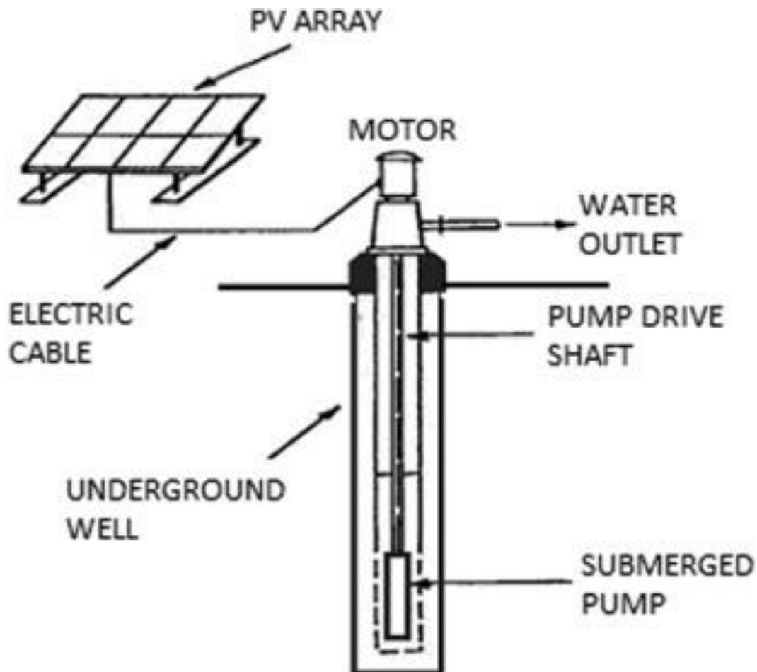
Fig. 1. Schematic of a simple PV irrigation set up for groundwater retrieval [6].
