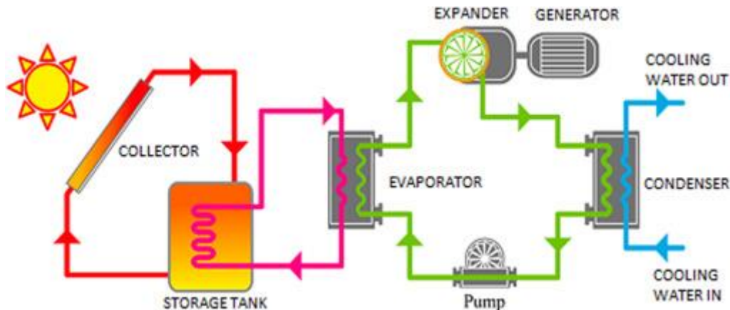
Fig. 13. Solar powered organic Rankine cycle system [66].
