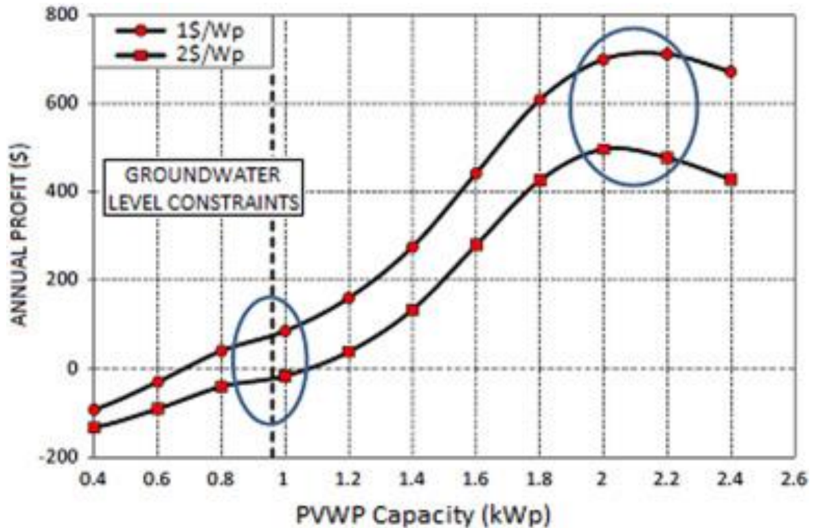
Fig. 5. Pump capacity vs annual profits with constrained groundwater levels [24].
