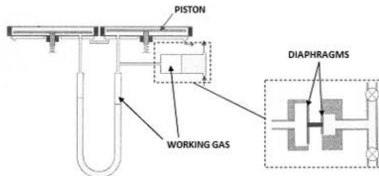
Fig. 11. Liquid Piston pump design using diaphragms [57].
