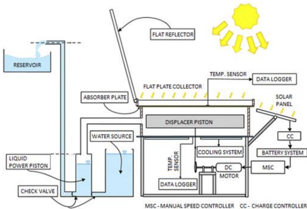
Fig. 15. Solar powered low temperature differential Stirling pump [72].
