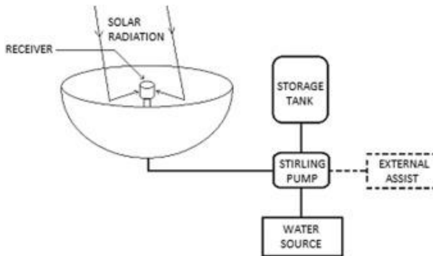
Fig. 19. Schematic of the most effective solar thermal water pumping system for remote rural areas based on literature reviews.
