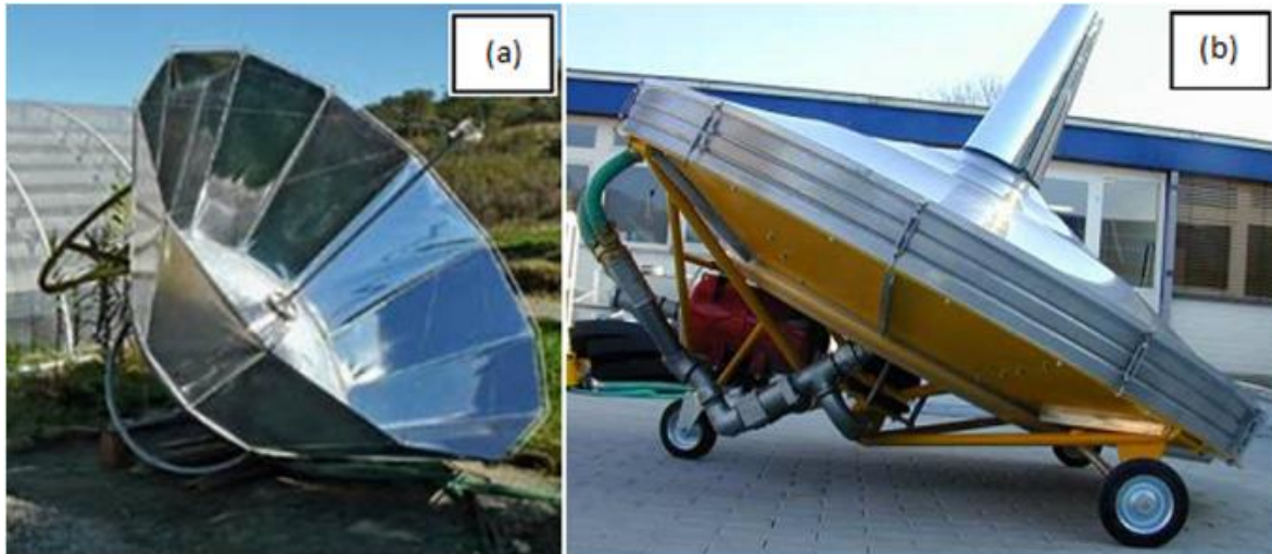
Fig. 20. (a) Solar Stirling water pump with dish [80] (b) SUNPULSE Stirling system [81].
