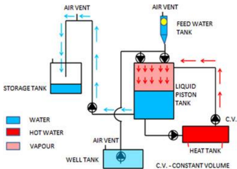
Fig. 17. 2-stroke liquid piston pump [69].
