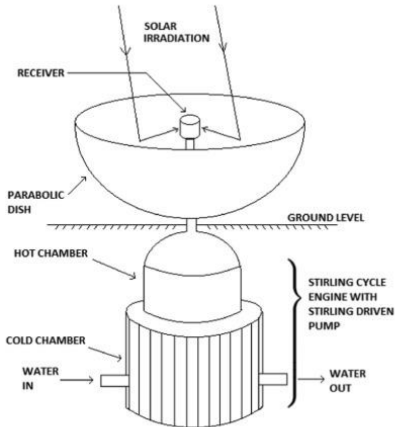
Fig. 10. An example of a Stirling cycle thermal power irrigation system.
